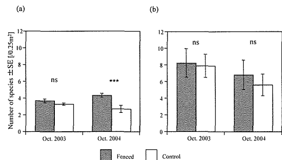
図-5 柵内外における群落構成種数 (a) 閉鎖林冠下の実験区 (b) 開放地の実験区 Fig.5 Species richness of in the fenced/control plots (a) plots under closed canopy (b) plots in open sites
