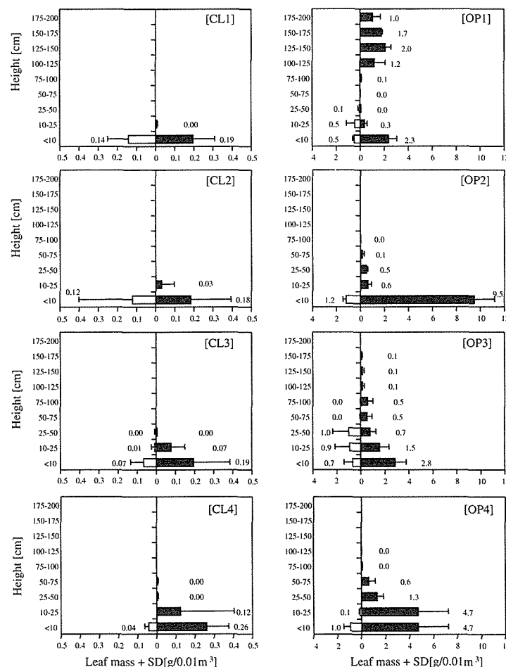
Fig.6 Vertical distribution of leaf biomass in each fenced and control plot
