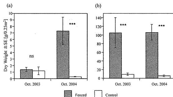
図-4 柵内外における群落現存量 (a) 閉鎖林冠下の実験区 (b) 開放地の実験区 Fig.4 Community biomass in the fenced/control plots (a) plots under closed canopy (b) plots in open sites
