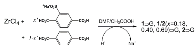
Scheme 1 Schematic for synthesis of ligand based solid solution frameworks.
