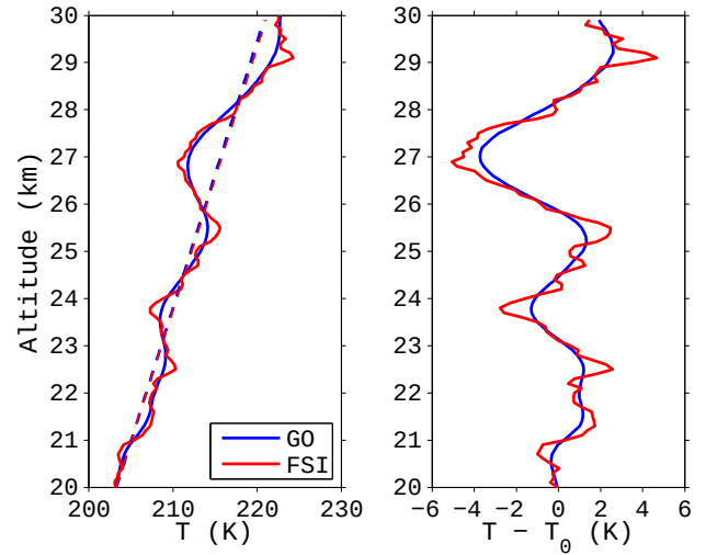
Figure 2. Atmospheric temperature profiles retrieved by GO (blue line) and FSI (red line) methods from COSMIC GPS-RO data obtained at 00:03 UTC on 1 January 2007 at 1.31° N and 136.265° E. The GO profile is obtained from CDAAC. Left panel shows the original temperature profiles with a linear fitting in dashed line. Right panel shows perturbation components (replotted from Tsuda et al., 2011).
