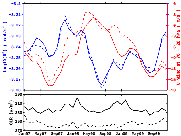
Figure 5. Time variations in N^2 (blue line) and U (red line) with positive eastward propagation in the tropics in the 20–27 km height range (top panel) and OLR (bottom). Solid and dashed lines correspond to the longitude regions (a) 90\text{--}150^\circ E and (b) 170\text{--}230^\circ E, respectively.
