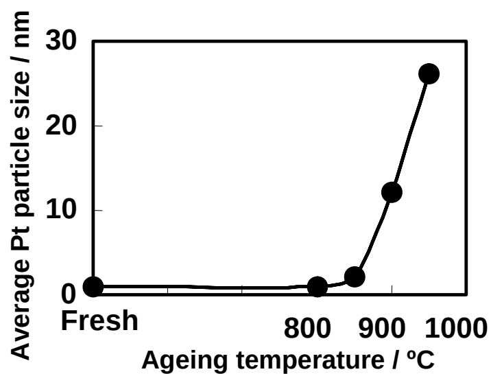
Figure 1. Average Pt particle size for aged Pt/ceria-based oxide catalysts at various temperatures under lean condition.
