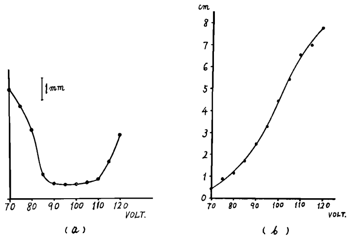
Fig. 19 Relations between voltage of electric source and deflection of galvanometer. (Relations between light intensity of projecting lamp and photo current.)
