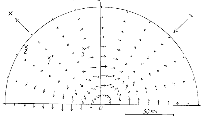
(C) Tilt.
