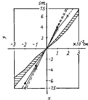
Fig. 15 Relation between movement ( x ) of iron core and deflection of galvanometer ( y ).
