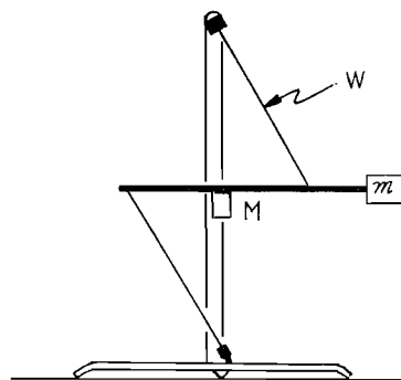
Fig. 5 Illustration of tiltmeter (horizontal pendulum). It is constructed mainly on super-invar. M: mirror, W: super-invar wire (50 \mu in diameter), m: mass.
