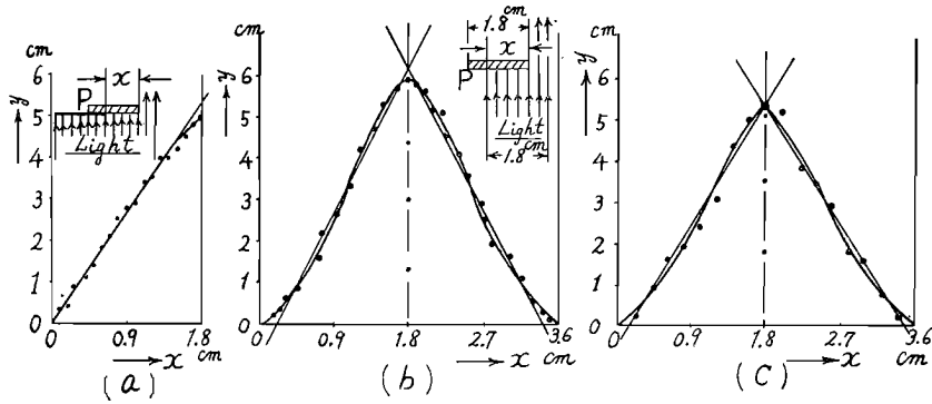
Fig. 18 Relations between exposed area on photocell and deflection of galvanometer (i.e. photo current).
