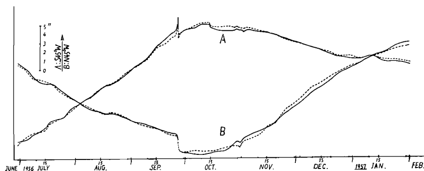
(b) Variation of ground-tilt observed with tiltmeter of horizontal pendulum type and photocell type, at Ide observatory.
