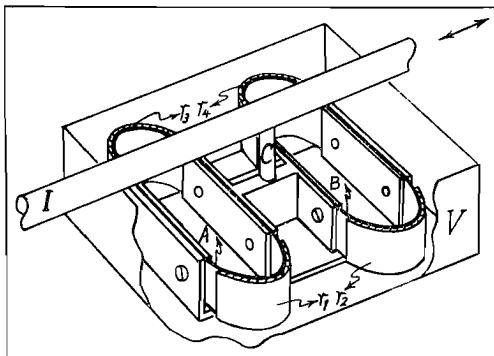
Fig. 12 Sketch of measuring gauges. (4 gauges method).
