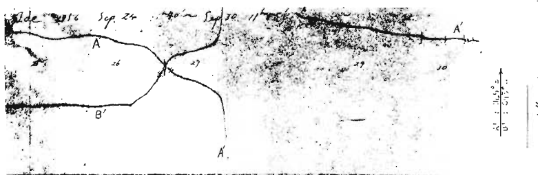
(C) Horizontal pendulum type tiltmeter (T.M.' A', B'). (Photographic recording).
