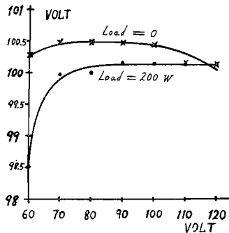
Fig. 17 Characteristic curve of voltage stabilizer.
