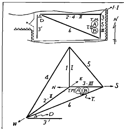
Fig. 4 Disposition of instruments interior the 1st observing room.
