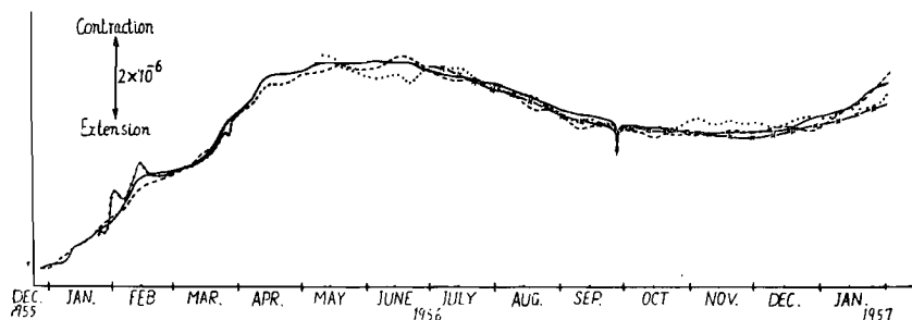
(a) Variation of strain observed with super-invar-bar extensometer, wire resistance strain meter, changing inductance type extensometer and photocell type extensometer, at Ide observatory.
