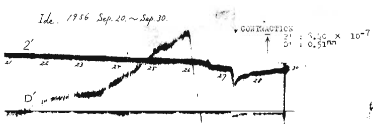
(B) Super-invar-bar extensometer (2') and discharge meter (D'). (Photographic recording).
