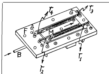
Fig. 13 Sketch of U_T -gauge.
