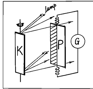
Fig. 10 Schematic view of photocell type instruments. K: mirror, P: photocell, G: galvanometer.
