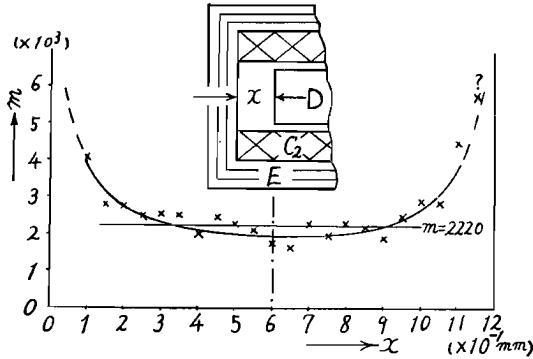
Fig. 16 Magnification curve of changing inductance type extensometer. (Magnetizing voltage of coil=32 V.)
