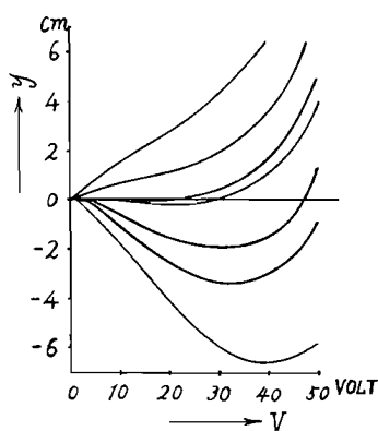
Fig. 14 Stability curve. (Relation between magnetizing voltage of coil and deflection of galvanometer.)
