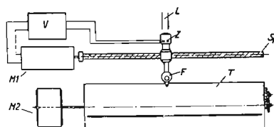
Fig. 22 Illustration of principle of photoelectric tracing recorder.
