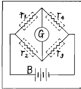
Fig. 9 Arrangement of gauges. (4 gauges r_1, r_2, r_3, r_4 : F-gauge, B: battery.
