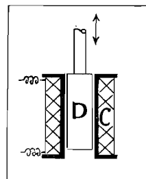
Fig. 8 Illustration of the changing inductance coil. C: coil, D: iron core.
