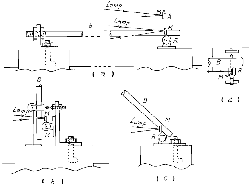
Fig. 3 Illustrations of super-invar-bar extensometers and high magnification extensometer.
