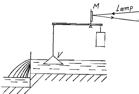
Fig. 6 Illustration of discharge meter. M: mirror, V: bouy.
