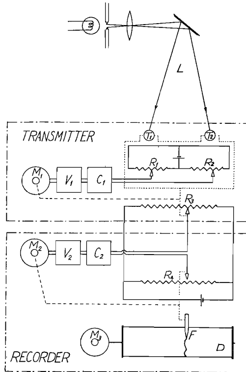
Fig. 21. Illustration of principle of tracing recorder with photo-transistor.
