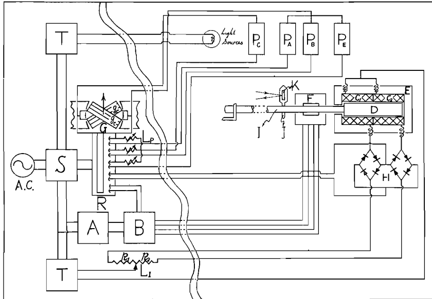
Fig. 11 Electric circuit of tele-metrical devices.
