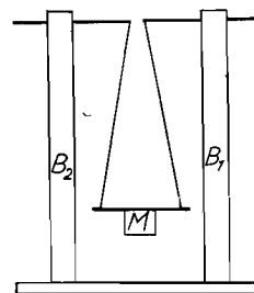
Fig. 7 Illustration of self-registering thermometer. M: mirror, B 1 ·B 2 : bimetal.
