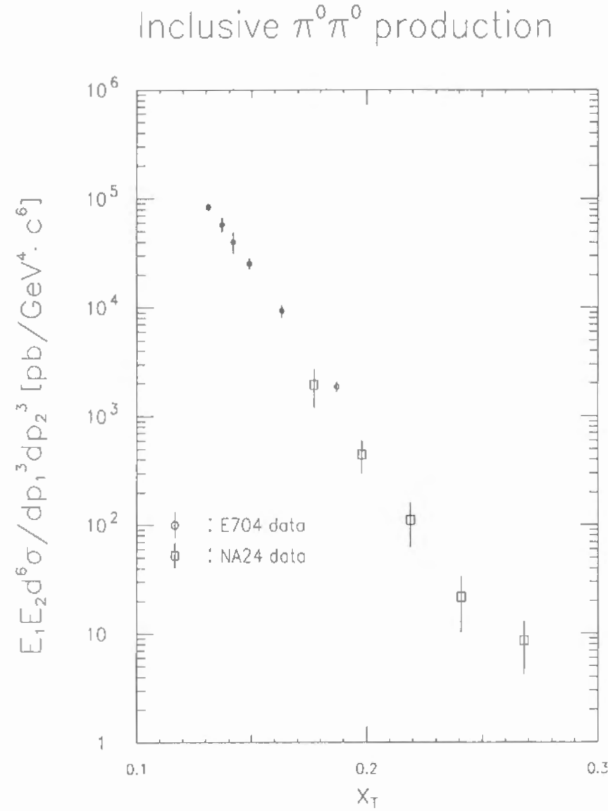
Fig.32: The invariant double-differential cross section for inclusive \pi^0\pi^0 production is compared to that from the NA24 results.
