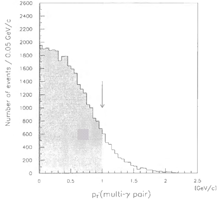
Fig.28: The p_T' distribution of multi- \gamma pair events in the M' region between 2.0 GeV/c and 2.1 GeV/c.
