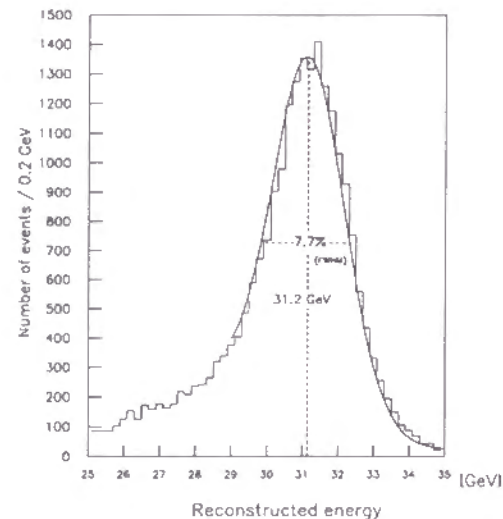
Fig.9: The reconstructed energy distribution with 31-GeV positron beam.
