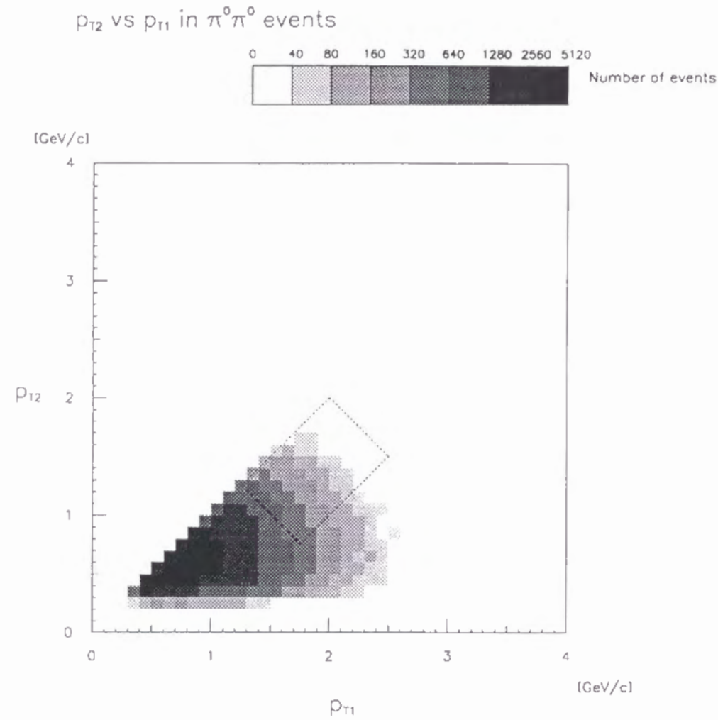
Fig.23: Relation between p_{T1} and p_{T2} in \pi^0\pi^0 events. The higher p_T of \pi^0 is defined as p_{T1} and the lower p_T of \pi^0 is defined as p_{T2} . The \pi^0\pi^0 events within the rectangle have been picked up for the analysis.
