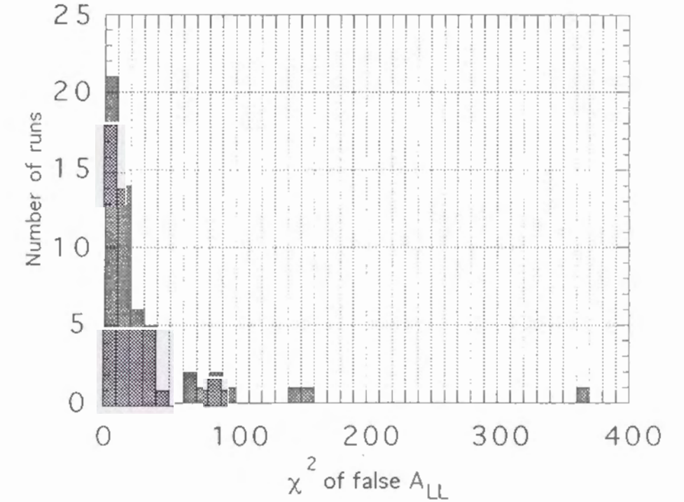
Fig.35: The \chi^2 distribution of the false A_{LL} for each run.
