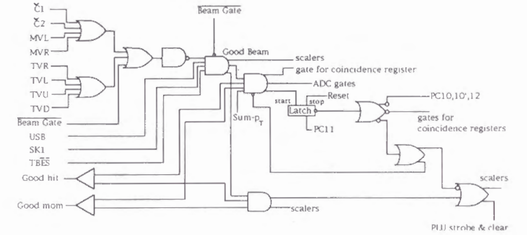
Fig.10: Scheme of the event trigger.
