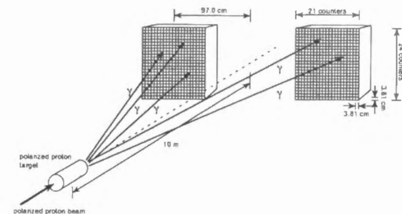
Fig.8: Schematic picture of CEMC1 and CEMC2.
