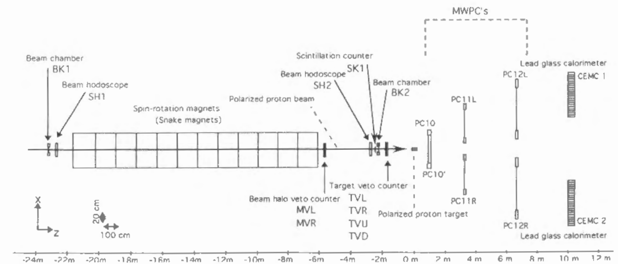
Fig.5: Vertical view of the experimental setup.
