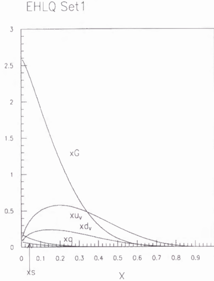
Fig.44: The distribution functions of valence u -quark, valence d -quark, strange quark, sea quark and gluon from the EHLQ set1.
