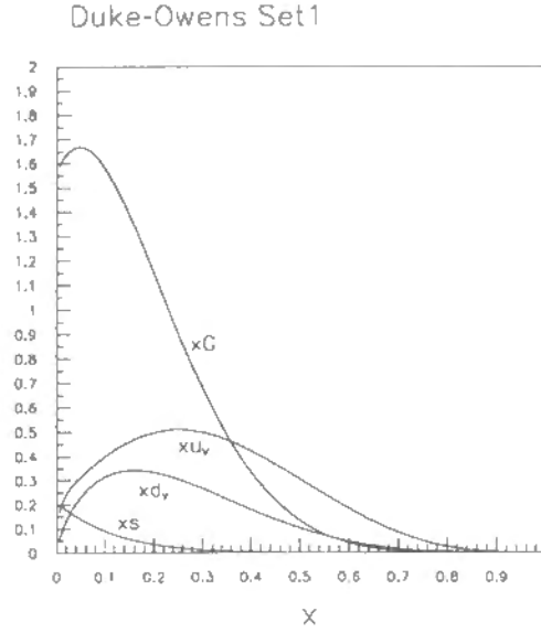
Fig.31: The distribution functions of valence u -quark, valence d -quark, sea quark and gluon from the Duke-Owens Set1.
