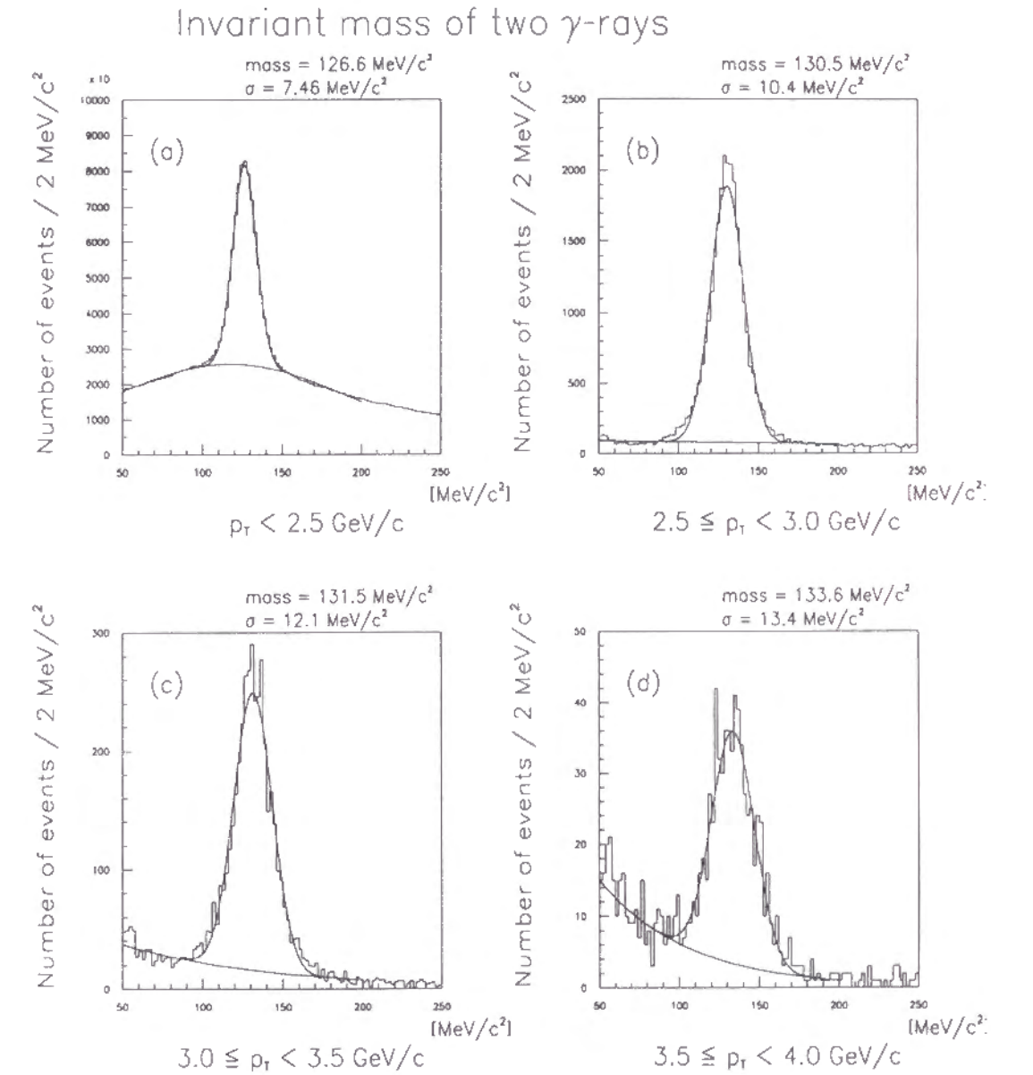
Fig.20: The distribution of invariant mass of \gamma -ray pairs for different p_T 's.
