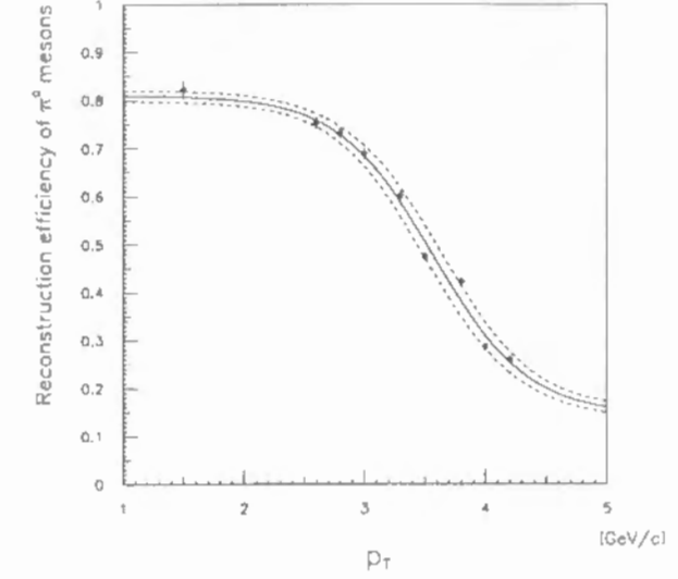
Fig.22: The p_T dependence of the reconstruction efficiency of \pi^0 .
