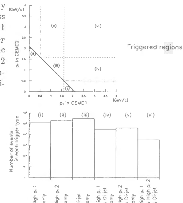
Fig.12: The relation among the "high p_T trigger" for CEMC1, the "high p_T trigger" for CEMC2 and the "di-jet trigger". The trigger rates for each region are shown in the histogram exclusively.
