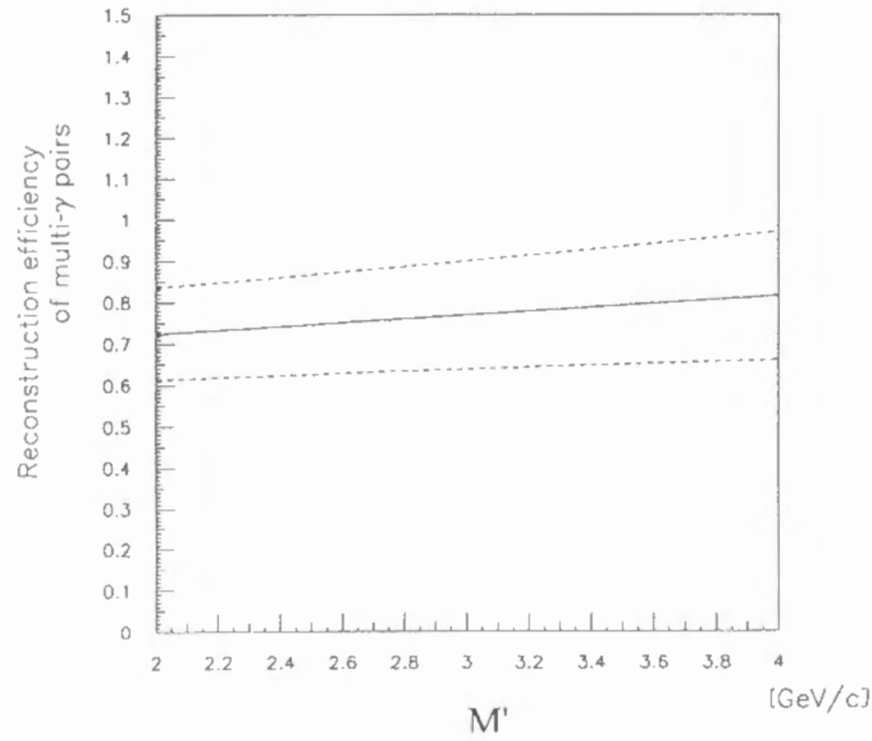
Fig.27: The reconstruction efficiency of multi- \gamma pair. (The dashed lines indicate the region of errors which comes from the fitting of input and reconstructed M' distribution.)
