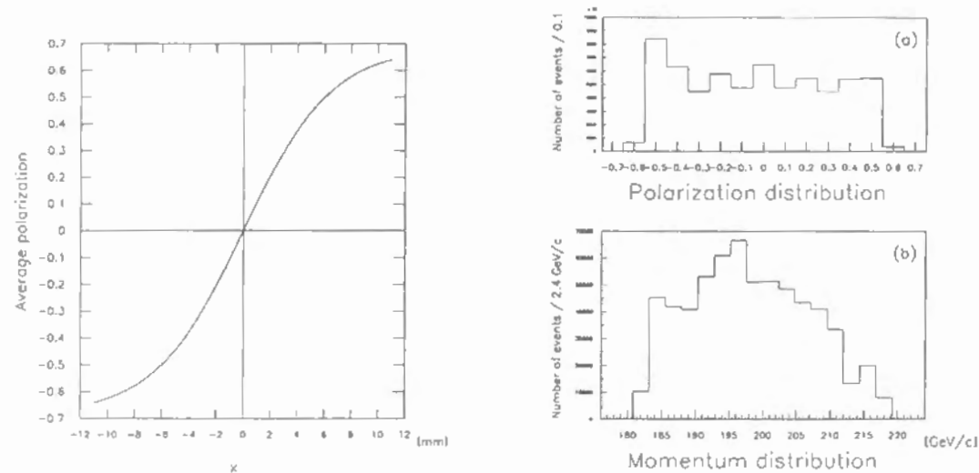
Fig.3: Correlation between the average particle polarization and the horizontal position at the middle of the polarized beam line (the tagging station).
