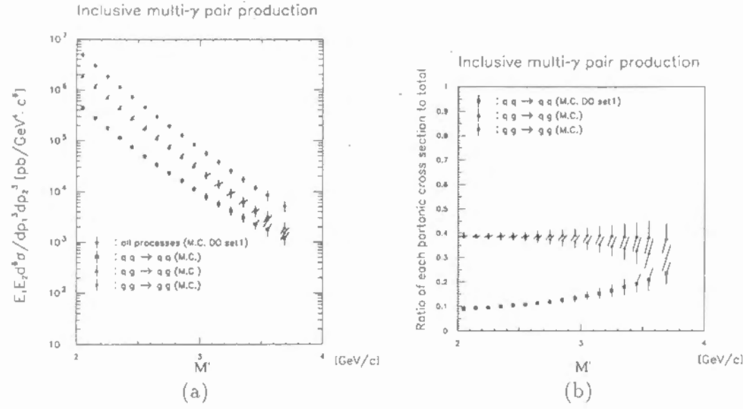
Fig.34: The contributions of gluon-gluon, gluon-quark and quark-quark scatterings to the inclusive multi- \gamma pair production obtained from the Monte-Carlo simulation with the Duke-Owens set1. The error bars indicate the statistical errors. (a) Invariant double-differential cross section for each partonic process (b) Contribution of partonic process to the total cross section
