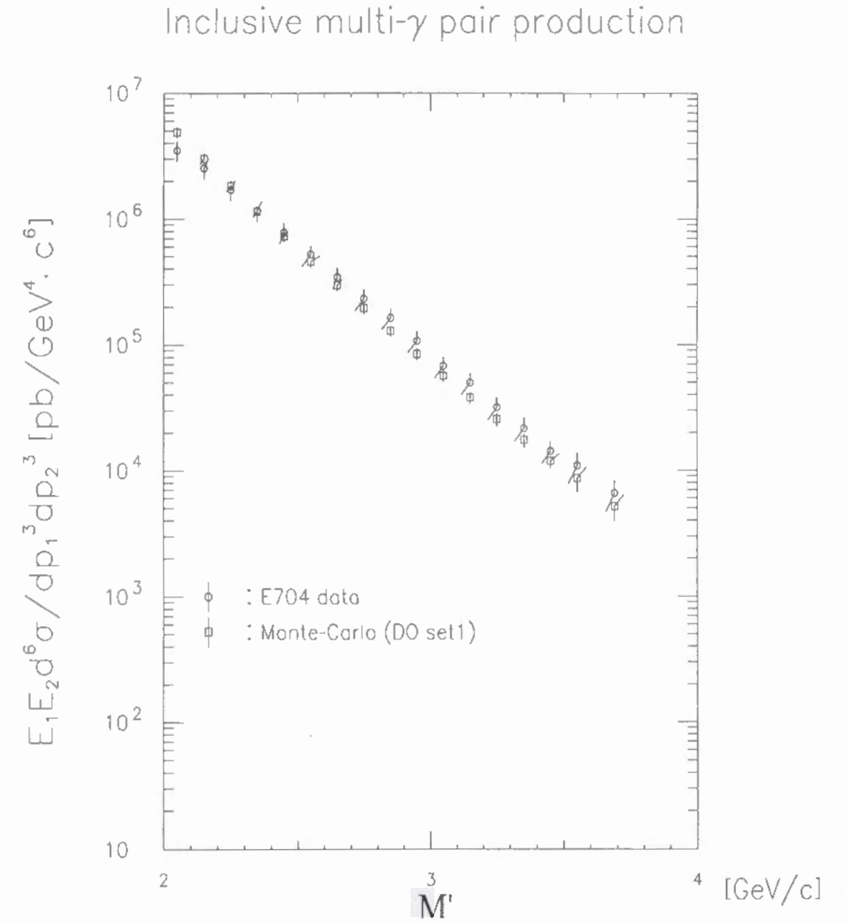
Fig.33: The invariant double-differential cross section for inclusive multi- \gamma pair production is compared to the Monte-Carlo results with the Duke-Owens Set 1.
