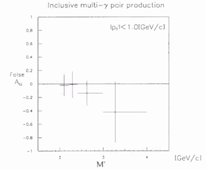
Fig.37: False A_{LL} for inclusive multi- \gamma pair production.
