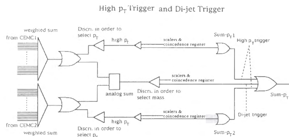
Fig.11: Scheme of the "high p_T trigger" and the "di-jet trigger".
