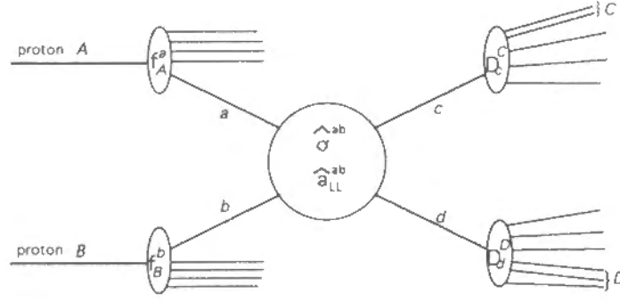
Fig.38: The parton picture of hard collision of protons. The partons a and b collide and create the partons c and d followed by fragmentation processes, D_c^C and D_d^D , to produce the final states C and D .
