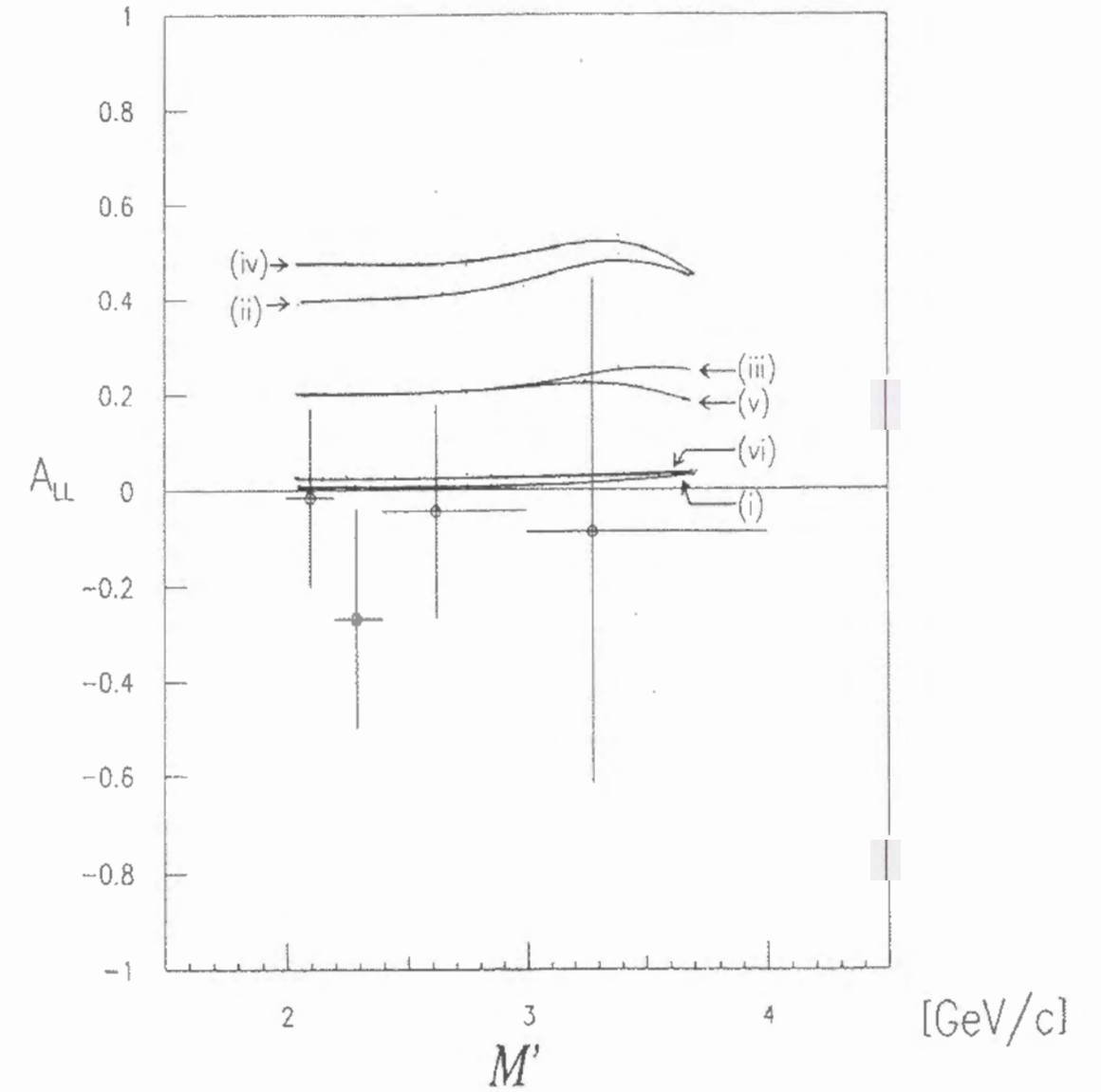
Fig.42: The theoretical calculations of A_{LL} compared with the present results. The \Delta G/G functions, (i), (ii), (iii), (iv), (v) and (vi), are used for the calculations.
