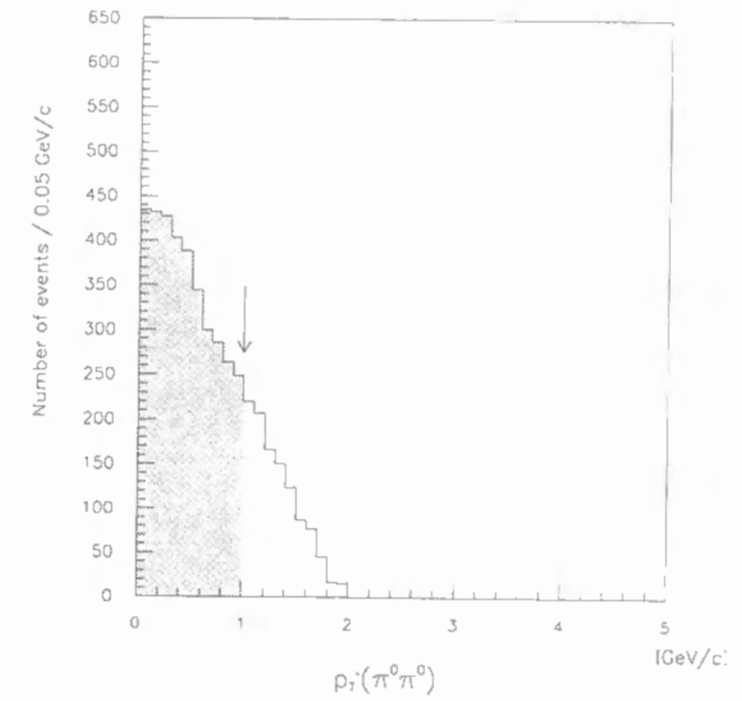
Fig.24: The p_{T'} distribution of \pi^0\pi^0 events in the M' region between 2.5 GeV/c and 2.6 GeV/c.
