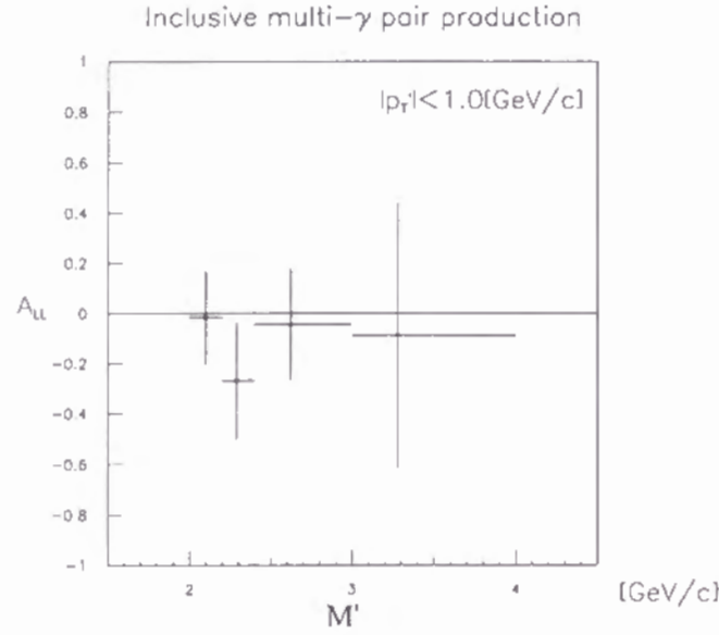
Fig.36: The A_{LL} for inclusive multi- \gamma pair production as a function of pseudo-mass, M' , with |p_T'| < 1.0 \text{ GeV/c} .
