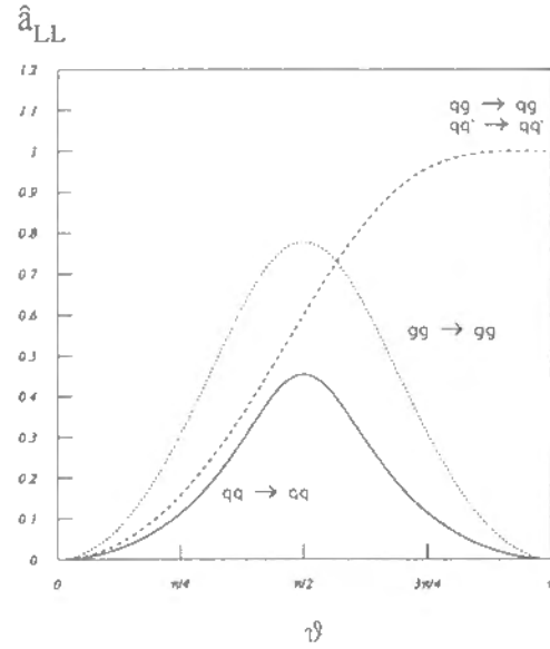
Fig.39: The double-helicity asymmetry, \hat{a}_{LL} , of the partonic processes, g + g \rightarrow g + g , q + g \rightarrow q + g , q + q \rightarrow q + q and q + q' \rightarrow q + q' .
