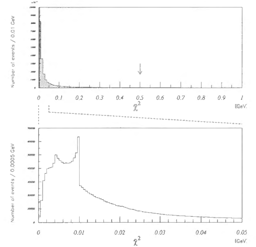
Fig.16: The \tilde{\chi}^2 distribution after the reconstruction of shower data. The magnified figure is shown below for the small \tilde{\chi}^2 region.
