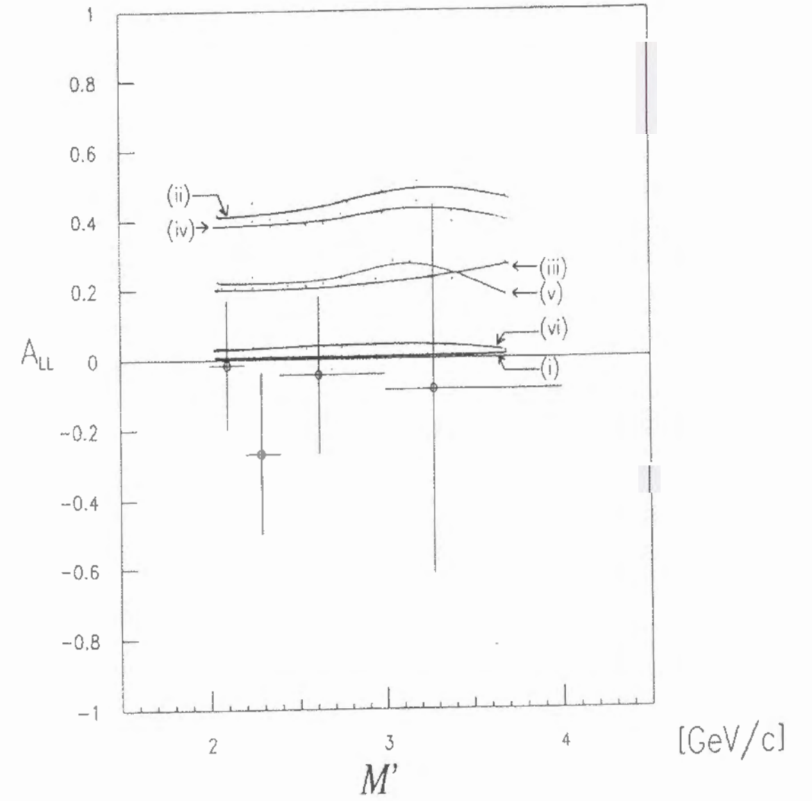
Fig.46: The theoretical calculations of A_{LL} with the EHLQ Set1 compared with the present results. The \Delta G/G functions, (i), (ii), (iii), (iv), (v) and (vi), are used for the calculations.
