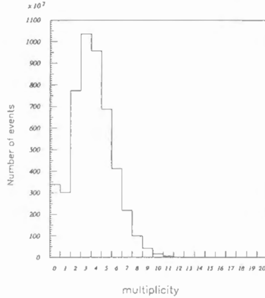
Fig.17: Multiplicity distribution of reconstructed \gamma -rays.
