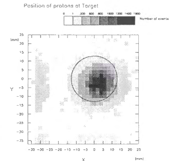
Fig.13: The hit positions of beam particles on the target reconstructed from the data of SH1 and SH2. The circle indicates the boundary of the target cut.
