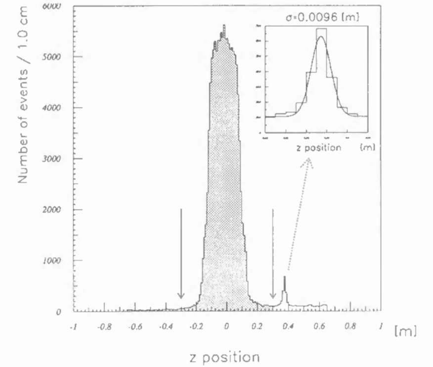
Fig.18: The distribution of z positions of event vertices reconstructed from the data of MWPC's. The events with the z vertex within \pm 0.3 m from the target center have been selected. At 0.37 m downstream the target, the peak came from the aluminum plate of 2 mm thick.
