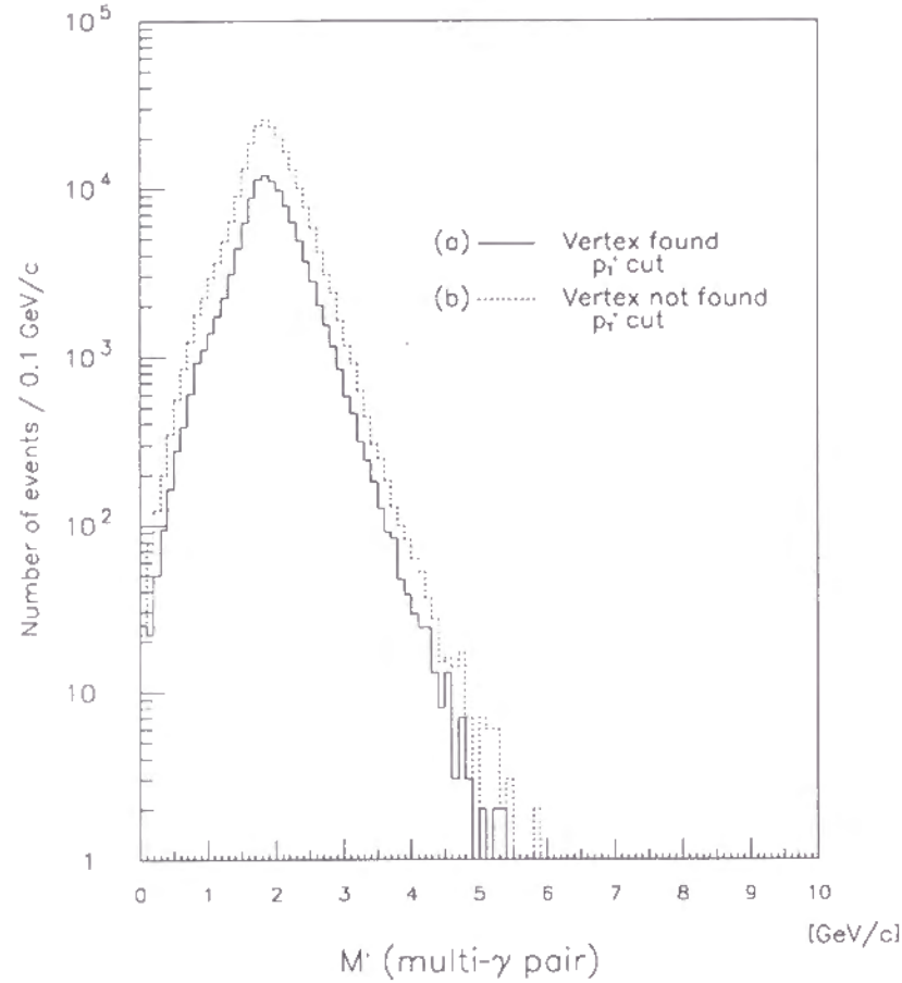
Fig.19: The M' distribution of the events for the following cases. (a) Vertex found from the MWPC data (b) No vertex found from the MWPC data
