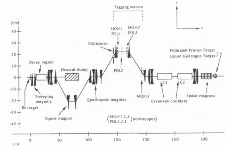
Fig.1: Schematic side view of the polarized proton beam line.
