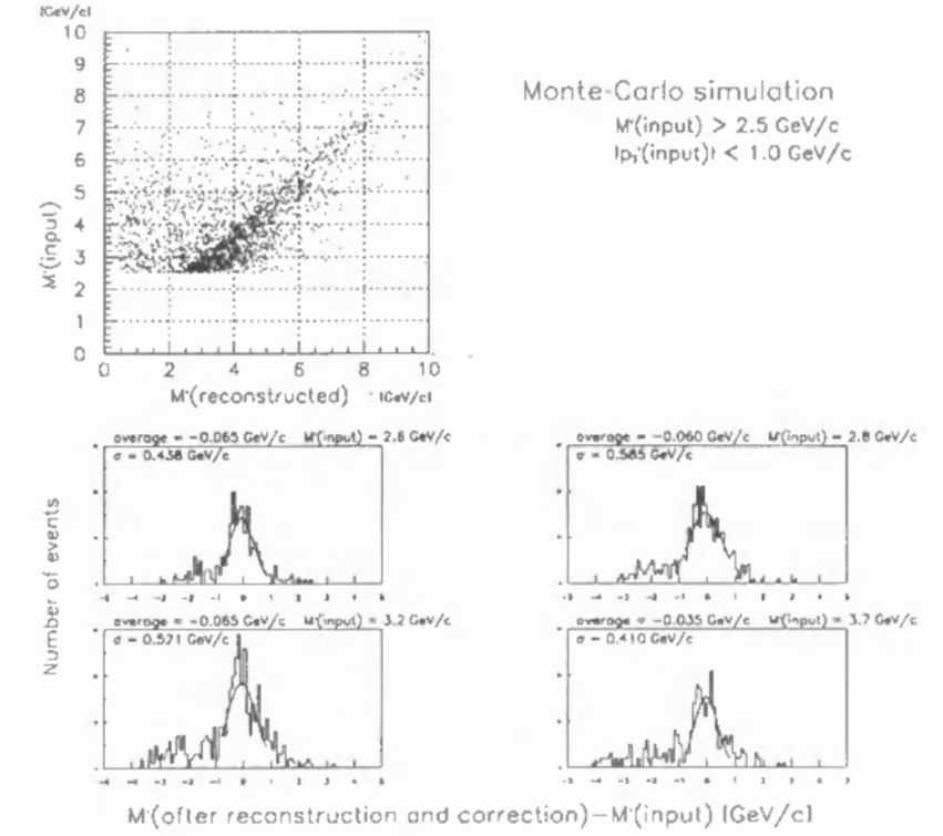
Fig.26: Relation between reconstructed M' and input M' from the Monte-Carlo simulation.
