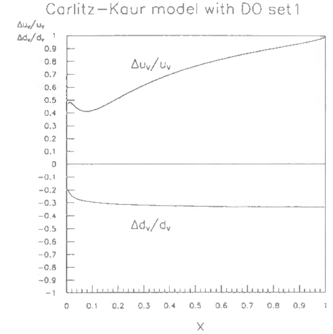
Fig.40: The polarization distributions of valence u -quark and d -quark obtained from the Carlitz-Kaur model with the Duke-Owens Set1.
