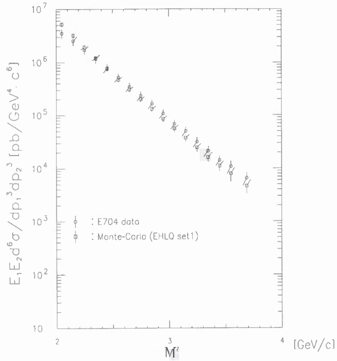
Fig.45: The invariant double-differential cross section for inclusive multi- \gamma pair production is compared to the Monte-Carlo results with the EHLQ Set1.
