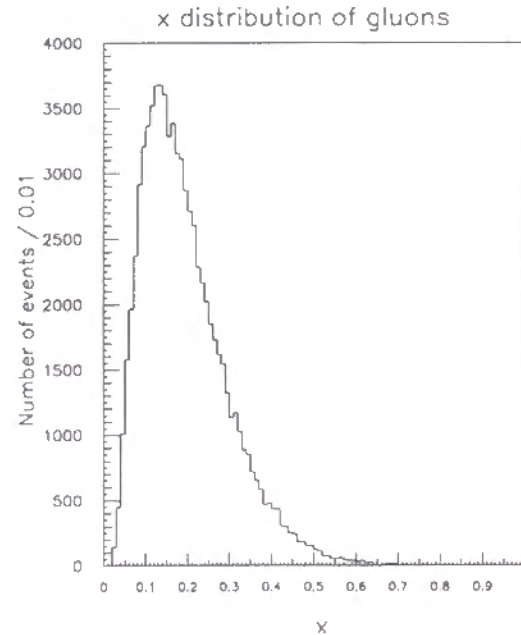
Fig.43: The x distribution of gluons which contribute to the multi- \gamma pair production, obtained by the Monte-Carlo simulation with the Duke-Owens Set 1.
