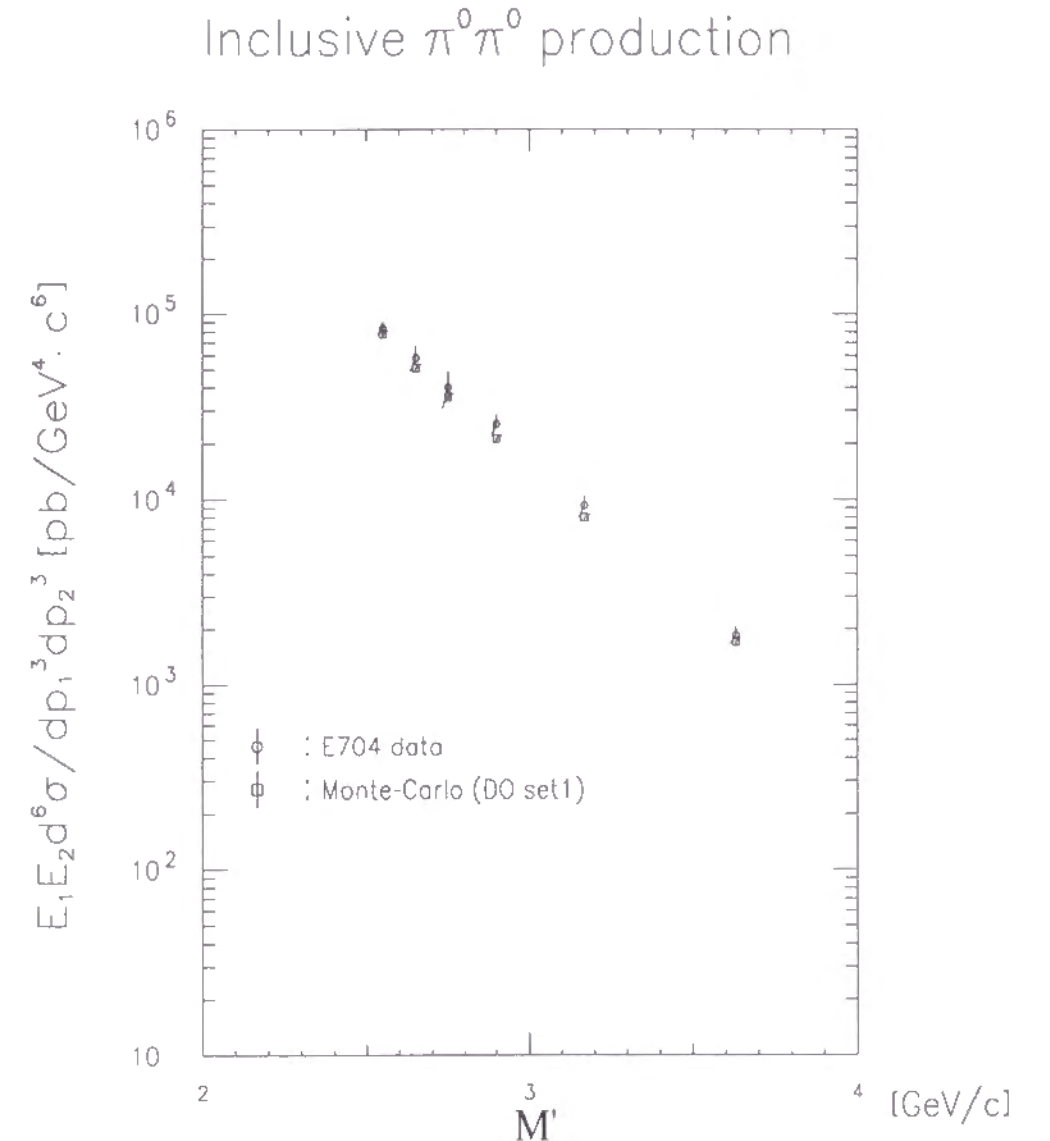
Fig.30: The invariant double-differential cross section for inclusive \pi^0\pi^0 production compared with the Monte-Carlo results with the Duke-Owens Set 1.
