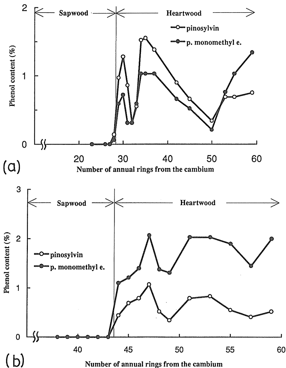
Fig. 4 Radial distribution patterns of pinosylvin and its monomethyl ether.
