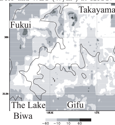
Fig. 10 The difference of latent heat fluxes between DRY and WET ( \text{W/m}^2 ) at 12JST.
