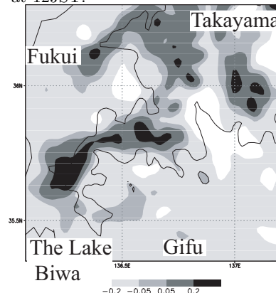
Fig. 12 The difference of precipitable water between DRY and WET ( \text{kg/m}^2 ) at 12JST.
