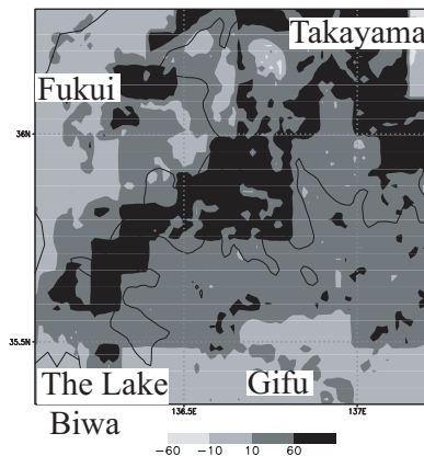
Fig. 9 The difference of sensible heat fluxes between DRY and WET ( \text{W/m}^2 ) at 12JST.
