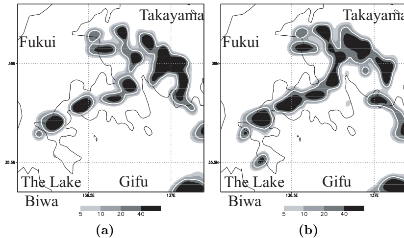
Fig. 7 Accumulated rainfall (mm) for 12JST - 18JST on 15th August 2001 with (a)WET, (b)DRY. The white thick line indicates accumulated rainfall of 20 mm and the black thick and thin lines indicate the terrain heights of 0m and 500m.
