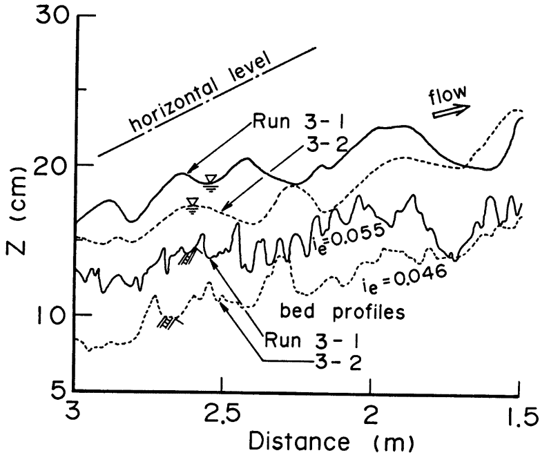
Fig. 11 Bed and water surface profiles appeared in the final stages of armouring processes. The profiles of Run 3-1 shows the final stage in the formative process of step-pool bed form, and on the other hand those of Run 3-2 indicates the final stage in the recreating process after the destruction of armour coat in Run 3-1.
