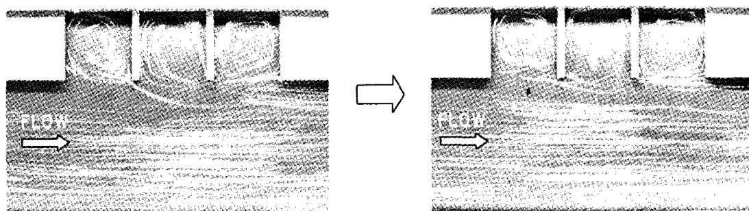
Fig. 11 Exchange process between the main channel and the embayment (inbank, B/W=2 )
