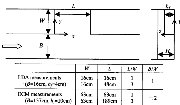
Fig. 1 Channel geometry and definition of dimensions
