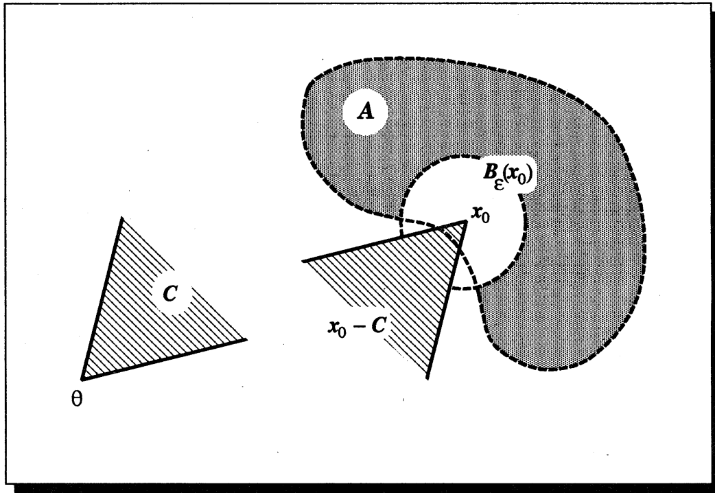
Figure 2.1: Illustration of a lower \varepsilon -approximately efficient point
