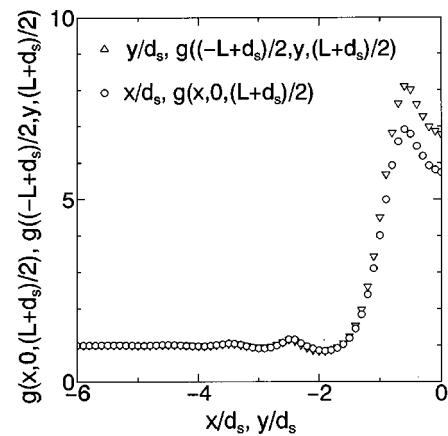
FIG. 5. The reduced density profiles of the small spheres, g(x, 0, (L + d_s)/2) and g((-L + d_s)/2, y, (L + d_s)/2) . A hard cube ( L = 2d_s ) without the cavity is considered as the solute. Since they are exactly symmetrical about x=0 and y=0 , respectively, the profiles are shown only for x \leq 0 and y \leq 0 . The step edge is located at x/d_s = -1 and y/d_s = -1 , respectively.
