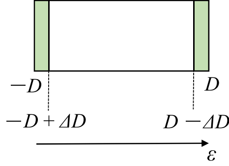
Figure 1.2: Schematic picture of the Anderson's poor-man's scaling method. The shaded regions mean the high-energy degrees of freedom (measured from the Fermi energy located at \varepsilon = 0 ) with the energy window \Delta D . Here 2D denotes the bandwidth of conduction electrons. By projecting out the high-energy degrees of freedom, we can obtain a low-energy effective theory composed of electrons at -D + \Delta D \leq \varepsilon \leq D - \Delta D .
