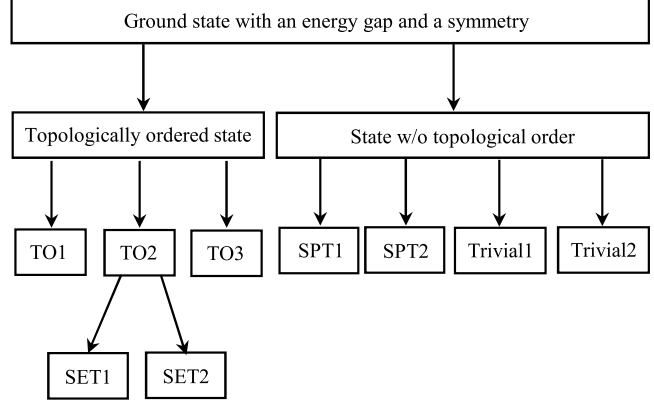
Figure 1.7: Classification of ground states with an energy gap. (a) The case where we do not assume any symmetry of the Hamiltonian and its deformation path. (b) The case where we assume some symmetry of the Hamiltonian and its deformation path. If the ground state breaks the symmetry of the Hamiltonian (which corresponds to the conventional Landau-Ginzburg-type order), the symmetry considered in the right panel is the unbroken symmetry which is retained by the ground state.
