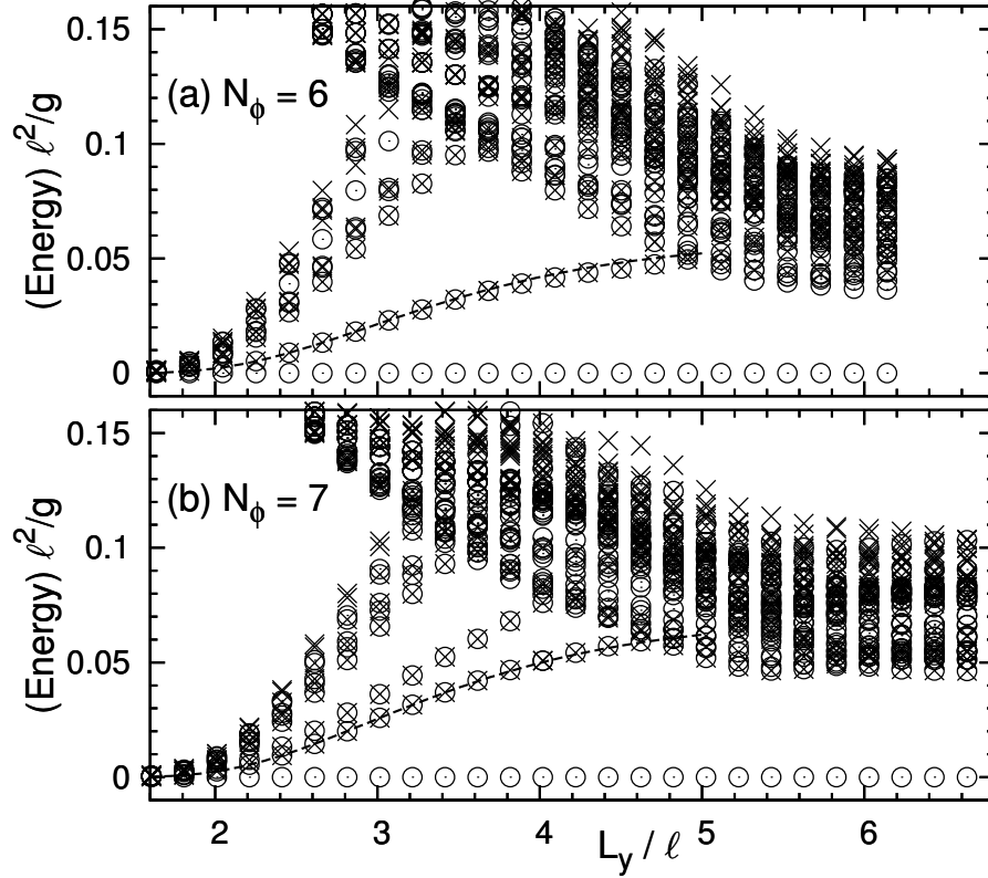
Figure 4.4: Energy spectrum of the Hamiltonian (4.4.3) as a function of L_y/\ell for (a) N_\phi = 6 and (b) N_\phi = 7 . The ground-state energy is subtracted from the spectrum. Circles indicate eigenenergies in the equal-population case N_1 = N_2 = N_\phi . Crosses indicates eigenenergies in the minimally imbalanced case (N_1, N_2) = (N_\phi + 1, N_\phi - 1) . The two lowest energies for each pseudomomentum are shown. The data for the largest L_y/\ell correspond to the case of L_x = L_y . Dashed lines indicate the energy gaps 0.721J and 0.857J of the spin-1 Heisenberg chain (4.4.11) with N_\phi = 6 and 7 spins, respectively, where J is given by V_{10} = 2V_{10}^{(12)} in Eq. (4.4.5) (we note that the gap in the thermodynamic limit [288, 289] is given by 0.410J ).
