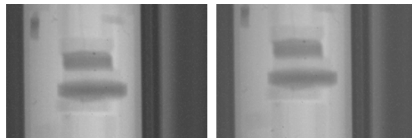
Figure 2 Radiography images of LiMn 2 O 4 / 7 Li-LATP / LiMn 2 O 4 symmetry cell after electrolyzed for (left) 1 h and (right) 3 h.
