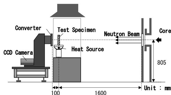
Fig. 1 Schematic diagram of the heating experiment.
