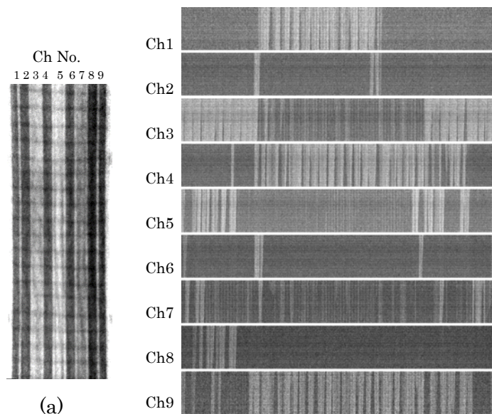
Fig.2 Visualization image ( x_{ex}=0.1 - G=50\text{kg/m}^2\text{s} ). (a) Time average image (b)Time strip image
