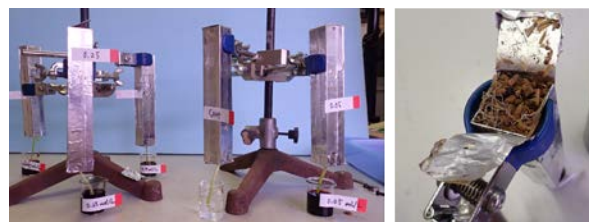
Fig. 1. Introduction of iodine solution into the sample. Left: at the time of introduction; Right: the bottom of the aluminum container is opened.
