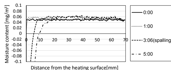
Fig. 2 Changes in the amount of moisture content.
