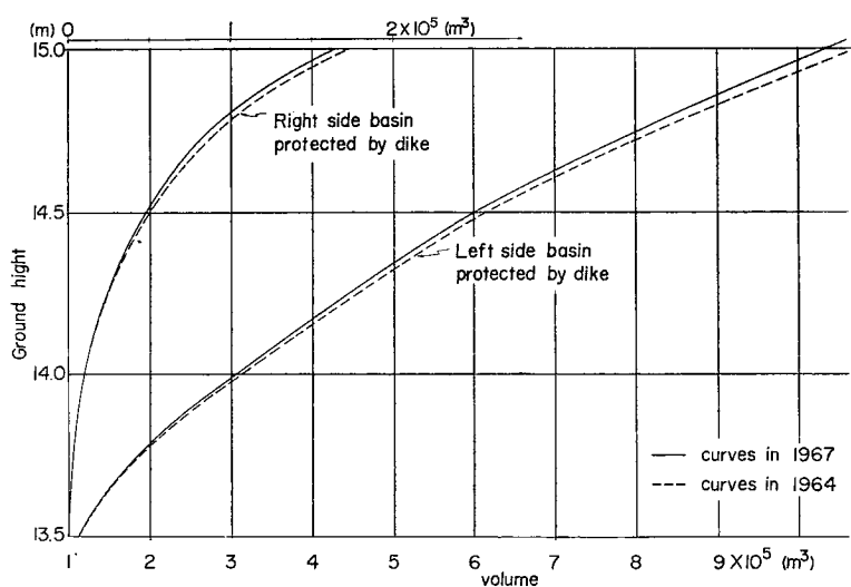
Fig. 3 H-V curves.
