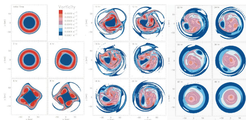
Fig. 2 The time evolution of vorticity field. Low vorticity values are shaded blue and high values are shaded red. (From Schubert et al. (1999))
