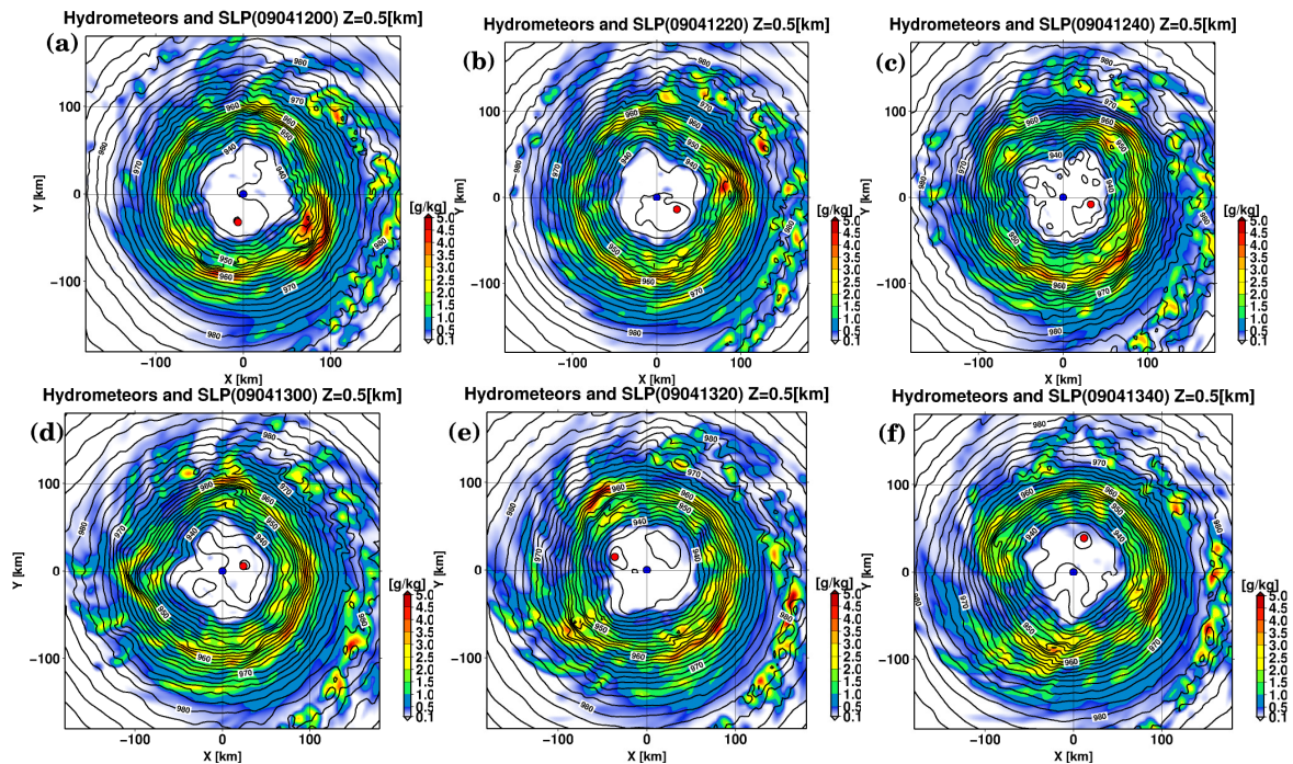
Fig. 6 Time evolution of the eyewall of simulated typhoon Songda. Shaded color denotes hydrometeors of cloud water, cloud ice, rain water and snow at a height of 0.5km. Contour line denotes sea level pressure. Blue circle denotes centroid center. Red circle denotes minimum pressure center. (a)1200UTC, (b)1220UTC, (c)1240UTC, (d)1300UTC, (e)1320UTC and (f)1340UTC.
