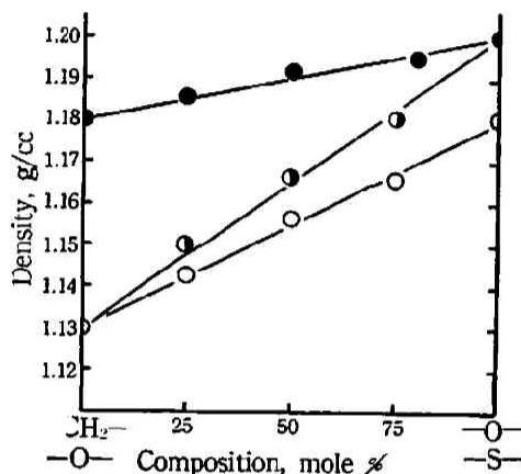
Fig. 4 Densities vs. composition in binary copolyamides ○ PXD-11/PXD-5O5, ◐ PXD-11/PXD-5S5, ● PXD-5O5/PXD-5S5
