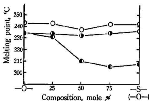
Fig. 3 Melting points vs. composition in copolyamides having both ether and thioether linkages and two different ether linkages ○ PXD-5O5/PXD-5S5, ◐ PXD-6O6/PXD-6S6, ● PXD-6O6/PXD-5O7
