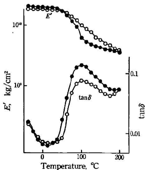
Fig. 6 Dynamic viscoelasticity of PXD-5O5 (undrawn) ○: Heat treated at 180°C
