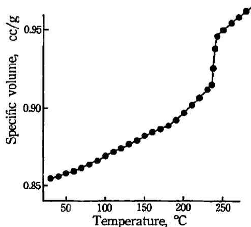
Fig. 5 Temperature-specific volume curve for PXD-5O5
