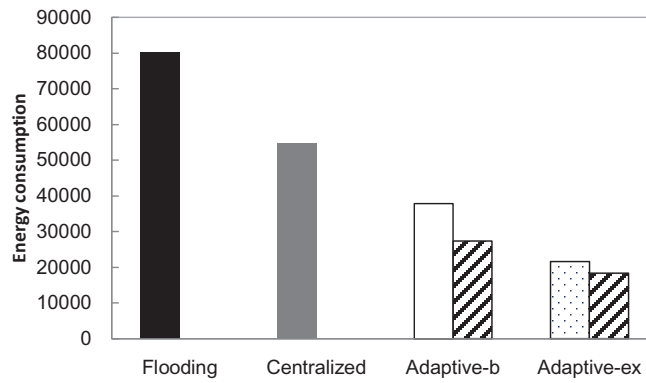
Fig. 2.7 Energy consumed in example 2.
