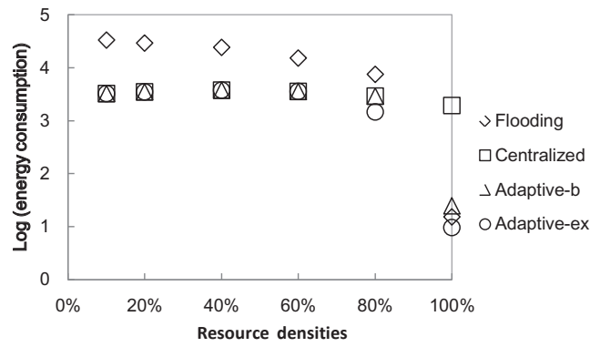
Fig. 2.10 Energy consumed under different resource densities.
