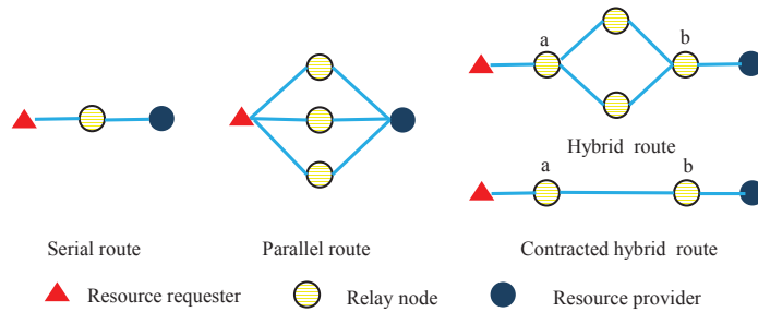
Fig. 3.4 Availability of routes.
