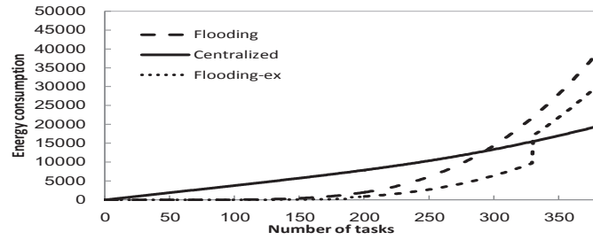
(c) 6 units of resources per node
