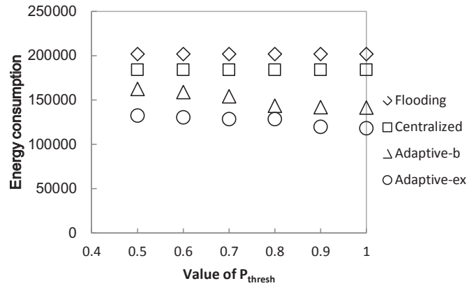
Fig. 2.12 Energy consumed with different values of P_{thresh} .
