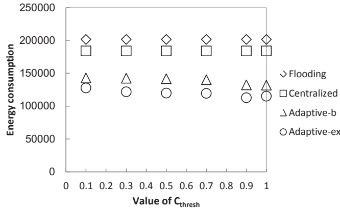
Fig. 2.11 Energy consumed with different values of C_{thresh} .
