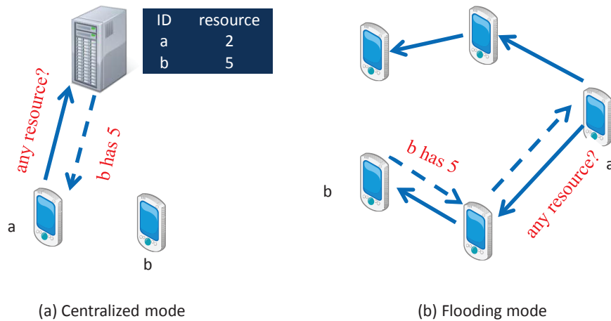
Fig. 1.3 Different strategies for resource discovery.
