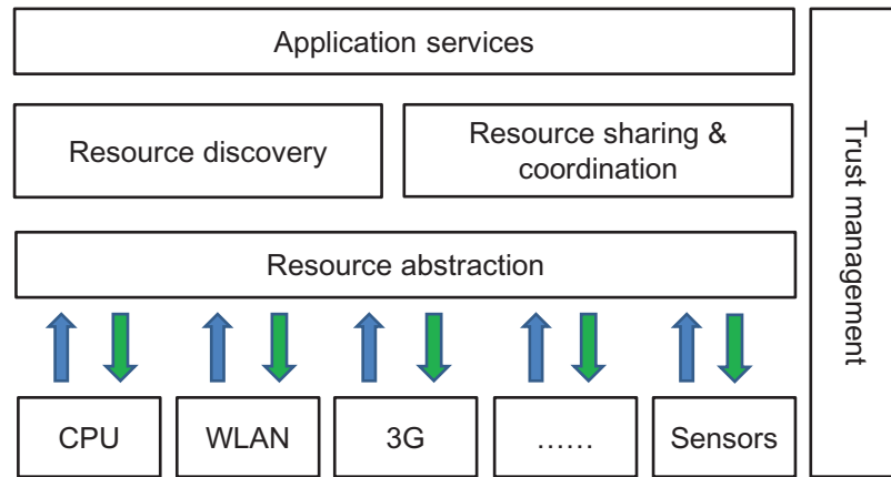
Fig. 1.2 Concept model of cooperative mobile cloud.
