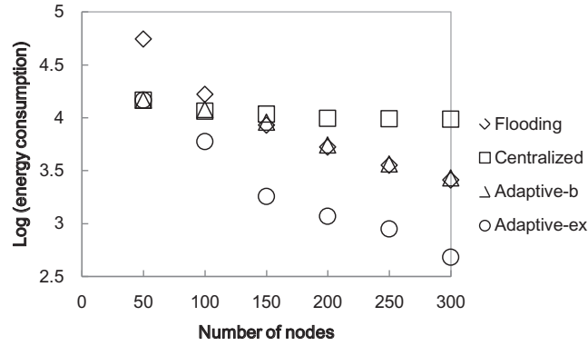
Fig. 2.9 Energy consumed under different node densities.
