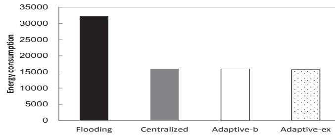
(b) Energy consumed in C-R
