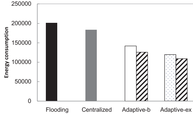
Fig. 2.6 Energy consumed in example 1.
