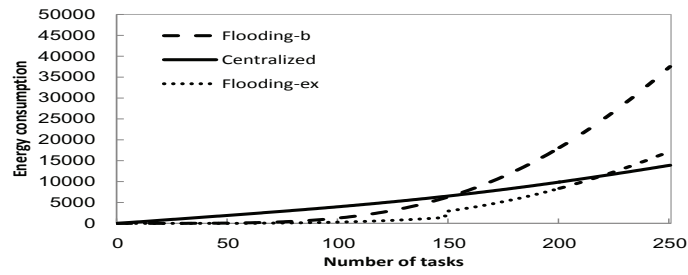
(b) 4 units of resources per node
