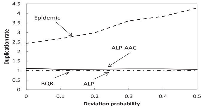
(b) Deviation probability
