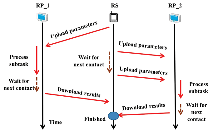
Fig. 4.2 Example flow of opportunistic resource sharing.
