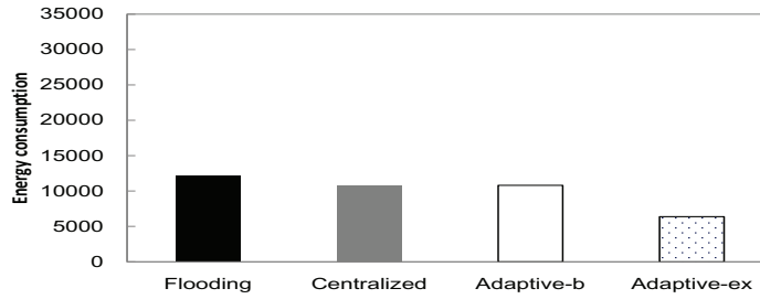
(c) Energy consumed in CR-R
