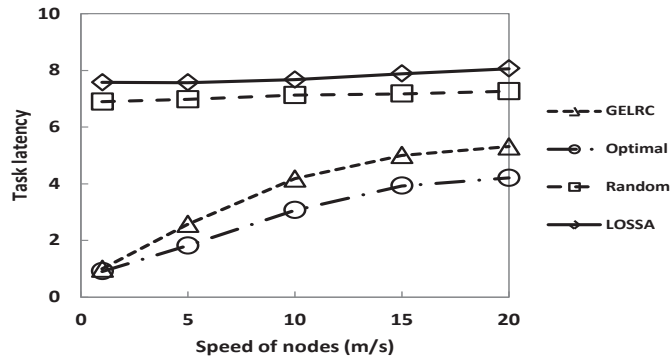
Fig. 3.6 Task latency of different methods.
