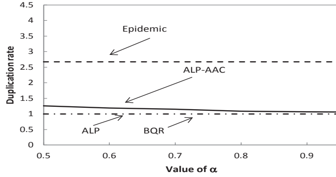
Fig. 4.8 Duplication rates for different values of \alpha .
