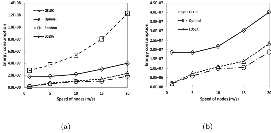
Fig. 3.5 Energy consumed by different methods.
