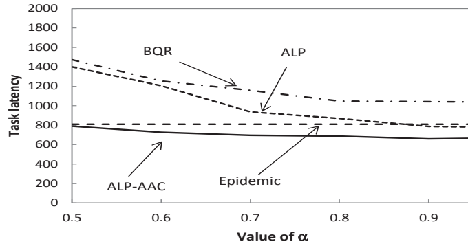
Fig. 4.7 Task latencies for different values of \alpha .
