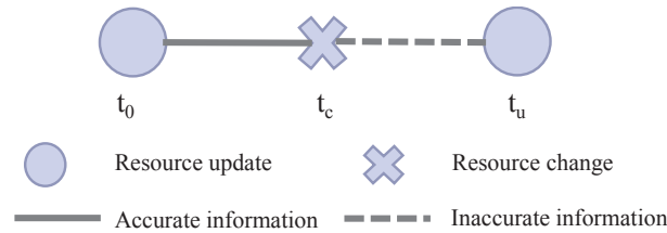
Fig. 2.3 Tradeoff in centralized mode.
