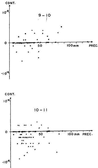
Fig. 7. Strain variations under the condition of the wet ground and that of the dry. \bigcirc shows the case of the wet and \times shows that of dry ground.
