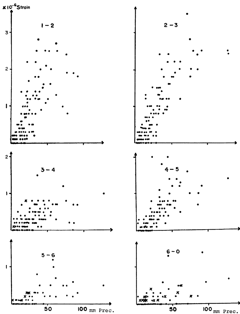
Fig. 5. Maximum amplitude verse rainfalls. \times shows extension and \bullet shows contraction. (a) Components in S34°E
