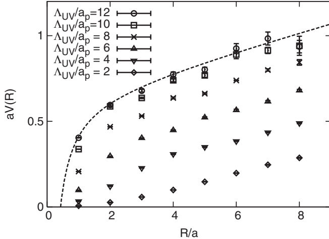
FIG. 2. The Q\bar{Q} potential with the UV cut \Lambda_{UV} plotted against the interquark distance R . The lattice QCD calculation is performed on 16^4 lattice with \beta = 6.0 . The unit is scaled with the lattice spacing, a \simeq 0.10 \text{ fm} or a_p \simeq 0.77 \text{ GeV} . The broken line is the original Q\bar{Q} potential in lattice QCD.
