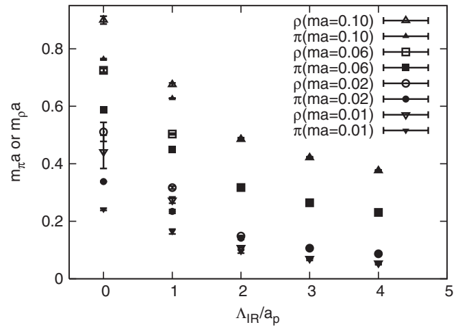
FIG. 9. The \Lambda_{IR} -dependence of meson masses with the staggered fermion. The bare current quark mass is taken as ma = 0.01, 0.02, 0.06 , and 0.10 . The unit is scaled with the lattice spacing, a \approx 0.10 fm or a_p \approx 0.77 GeV.
