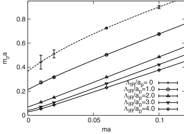
FIG. 10. The rho mass m_\rho plotted against the bare current quark mass m in the staggered fermion action. Chiral extrapolation is performed with (m_\rho a)^2 = c_2(ma)^2 + c_1(ma) + c_0 . The data with \Lambda_{\text{IR}} = 0 (broken line) is the standard lattice result. The unit is scaled with the lattice spacing, a \simeq 0.10 fm or a_p \simeq 0.77 GeV.
