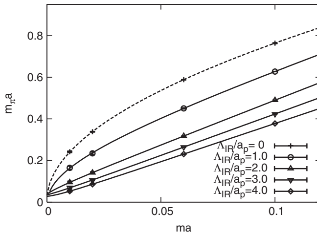
FIG. 11. The pion mass m_\pi plotted against the bare current quark mass m in the staggered fermion action. The notation is the same as Fig. 10.
