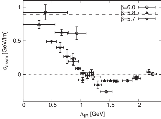
FIG. 5. The \Lambda_{\text{IR}} -dependence of the asymptotic string tension \sigma_{\text{asym}} in physical unit. The notation is the same as that used in Fig. 4.
