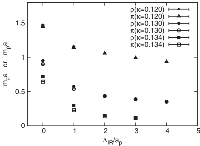
FIG. 8. The \Lambda_{IR} -dependence of meson masses with the clover fermion. The data at \Lambda_{IR}/a_p = 0 is the standard lattice result. The notation is the same as Fig. 7.
