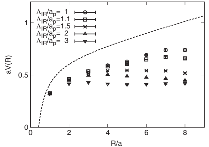
FIG. 3. The Q\bar{Q} potential V(R) with the IR cut \Lambda_{IR} . The notation is the same as Fig. 2.
