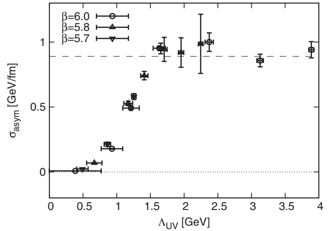
FIG. 4. The \Lambda_{\text{UV}} -dependence of the asymptotic string tension \sigma_{\text{asym}} in physical unit. The vertical error bar is the standard statistical error, and the horizontal error bar is the range that yields the same result due to the discrete momentum. The original value of the string tension is \sigma \simeq 0.89 GeV/fm (broken line).
