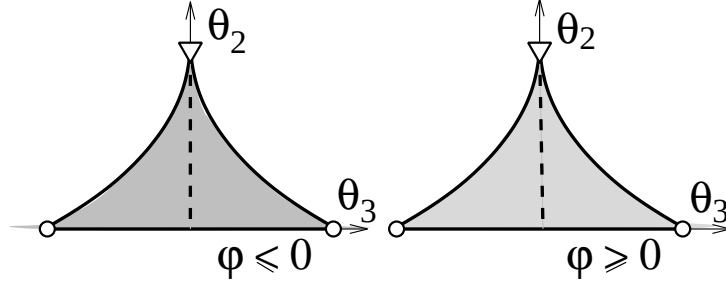
Figure 12: Degeneracy points on the space of orbits. Dash line corresponds to six-point degeneracy orbits with C_1 stabilizer. Two-point orbit with C_3 stabilizer is represented by a triangle. Two three-point orbits with C_2 stabilizer are shown by circles. Note that the respective points on the boundary of \varphi \leq 0 and \varphi \geq 0 domains should be identified. (See figure 5.)
