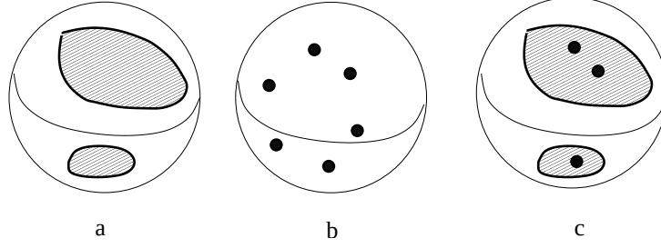
Figure 2: Schematic description of generic situations for regular domains. a) - Description on the sphere of regions with a_{11} - a_{22} \geq 0 . Hatched region - positive values. Boundary black curve - zero value. b) - Solutions of a_{12} = b_{12} = 0 . - isolated black points. c) - Description of the regular U_{\text{up}} domain. Only black points (which belong to hatched regions) should be excluded from the sphere to get the open set U_{\text{up}} .
