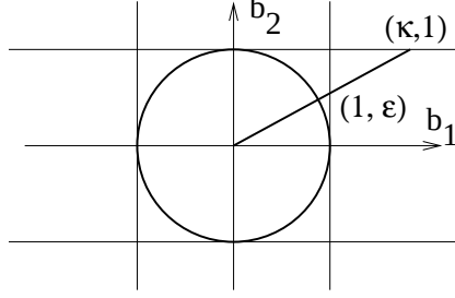
Figure 17: Local coordinate patches (B).
