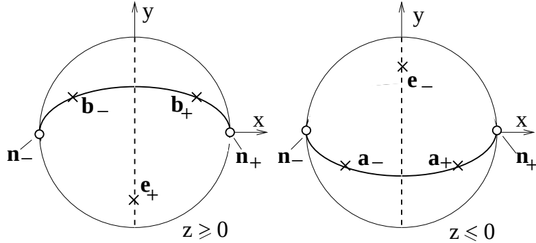
Figure 18: Positions of exceptional points on the sphere along the closed path 1 represented in Fig. 15. The sphere is shown through projections of its north ( z \geq 0 ) and south ( z \leq 0 ) hemispheres on the plane \{x, y\} . The \mathbf{n}_+ and \mathbf{n}_- as exceptional points are fixed and present for all points along the path 1 . Positions of \mathbf{e}_+ and \mathbf{e}_- exceptional points are shown by dash line. The \mathbf{e}_+ = -\mathbf{e}_- move along the great circle. Projections of the points \mathbf{a}_{\pm}, \mathbf{b}_{\pm} on the \{x, y\} plane move along ellipsoidal curve shown by solid line. These four points appears by bifurcating from \mathbf{n}_{\pm} points at \kappa = -9/4 and disappears through bifurcation at \kappa = 27/100 at x = 0 point of the solid curve.
