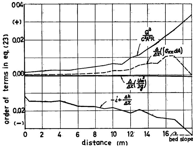
Fig. 9 (a) The order of terms in eq. (23) of profile in Fig. 2 (ii)
