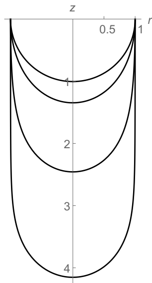
Figure 1. Black droplet solutions for fixed horizon radius at the boundary ( r_b = 1 ) and varying surface gravity \tilde{\kappa} . The AdS boundary z = 0 is at the top, and z increases towards the bottom. The solutions correspond to \lambda = 2\tilde{\kappa}r_b = 0.01, 0.5, 0.95, 0.9995 , with the elongation growing as \lambda increases towards 1.
