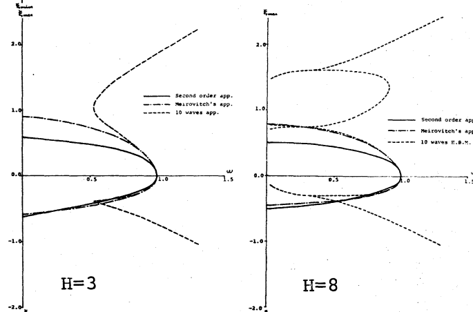
Fig.11: Backbone Curves by Perturbation Method (No.3)
