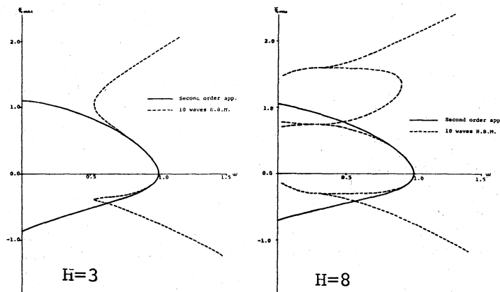
Fig.8: Backbone Curves by Bogoliuboff-Mitropolsky's Asymptotic Method
