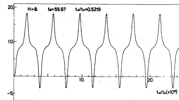
Fig.6: Waveform in H=8
