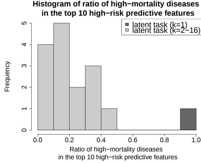
Fig. 4.4: Histogram of the ratio of high-mortality diseases in the top-10 high-risk predictive features. For a latent task ( k = 1 ), the highest-risk predictive features are composed of high-mortality diseases, whereas this tendency is not observed for other latent tasks.
