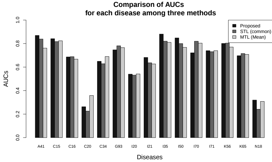
Fig. 3.3: Comparison of AUCs for each disease among the Proposed, STL (common), and MTL (Mean) methods in the prediction setting of day 1.
