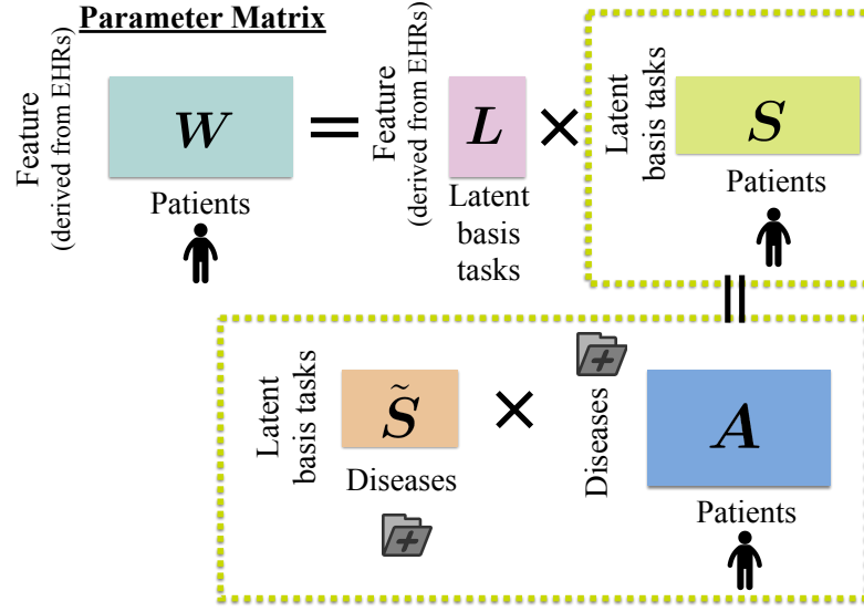
Fig. 4.2: Our MTL model for patients with multiple diseases.
