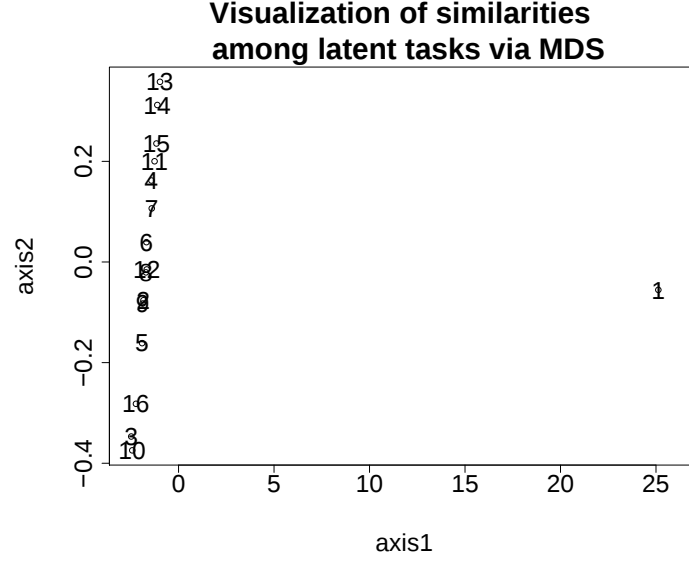
Fig. 4.3: Visualization of similarities among latent tasks via MDS using \tilde{S} . Only one latent task ( k = 1 ) was positioned as an outlier, while all others aligned with one dimension.
