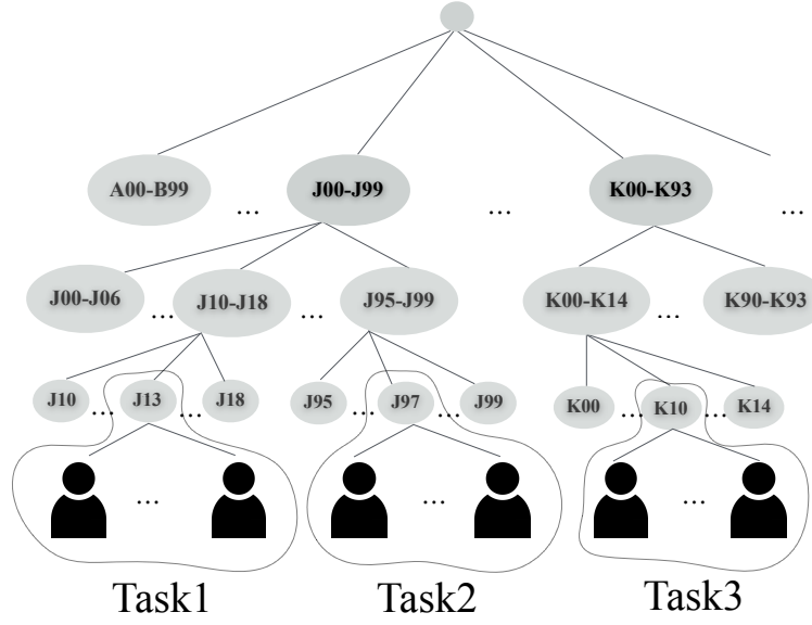
Fig. 3.2: An example of multitask learning formulation for multiple disease types. Patients are grouped into a task by their main disease as defined by the third level of the ICD-10 hierarchy. We define the similarities among diseases from this hierarchical structure to jointly learn prediction models for different diseases via multitask learning.
