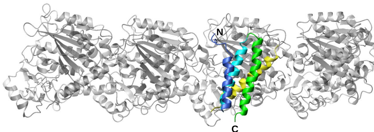
FIGURE 11. Model of \alpha -tubulin binding with kp60-NTD. Ribbon diagram of a model complex between kp60-NTD and a tubulin tetramer ( gray ) is shown. \alpha -Tubulin helix 12, a putative interface of kp60-NTD, is colored yellow .
