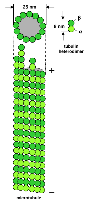
FIGURE 1. MT structure. Head-to-tail interactions of \alpha\beta dimers form linear protofilaments. 13 protofilaments associate laterally to form hollow cylindrical polymers.
