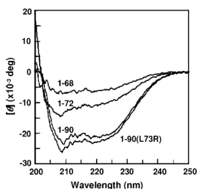
FIGURE 6. Comparison of CD spectra of kp60 N-terminal domains. N-terminal domain variants are shown in the panel. Each 10 \mu M of protein were dissolved in buffer containing 1 mM EDTA and 50 mM Tris-HCl (pH 7.5)
