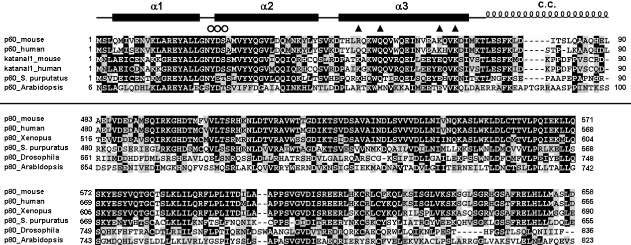
FIGURE 1. Domain architectures and multiple sequence alignment of p60-katanin and adaptor-p80. (A) Domain architectures of mouse p60-katanin and adaptor-p80. The regions of interaction between each domain are indicated by an arrow. vMIT, variant MIT domain; c.c., coiled-coil; AAA, AAA domain; CTD, C-terminal domain. (B) Multiple sequence alignment of p60-vMIT and p80-CTD, which interact with each other. The secondary structure elements of p60-vMIT are shown at the top. Filled triangles indicate residues involved in tubulin binding. Open circles indicate residues involved in \text{Ca}^{2+} binding (see Fig. 9). The protein names and UniProtKB accession numbers are as follows: p60 mouse (Q9WV86), p60 human (O75449), katanal1 mouse (Q8K0T4), katanal1 human (Q9BW62), p60 Stroglyocentrotus purpuratus (O61577), p60 Arabidopsis (Q9SEX2), p80 mouse (Q8BG40), p80 human (Q9BVA0), p80 Xenopus (Q4V7Y7), p80 Stroglyocentrotus purpuratus (O61585), p80 Drosophila (Q9NHF0), and p80 Arabidopsis (Q8H0T9). The sequence alignment was generated by ClustalX 45 .
