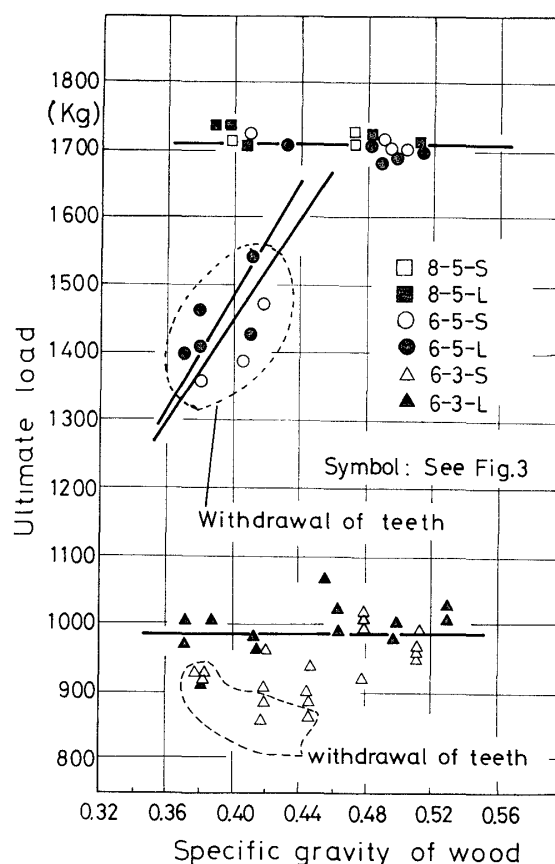
Fig. 12. Ultimate load of joints with six and eight rows types plate connectors as a function of specific gravity of wood.
