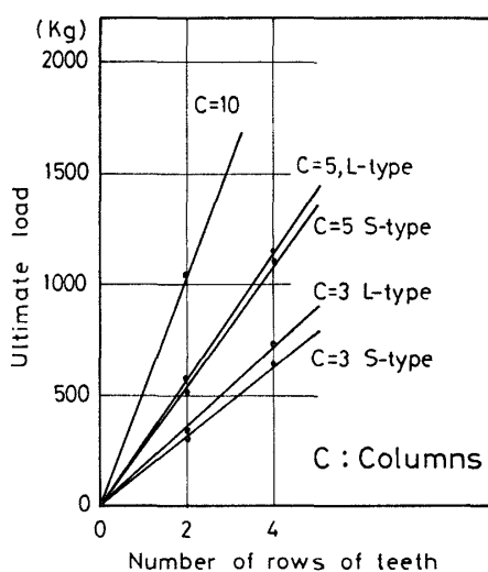
Fig. 11. Relation between ultimate load and number of rows of teeth of plate connectors. (Specific gravity of wood=0.40)
