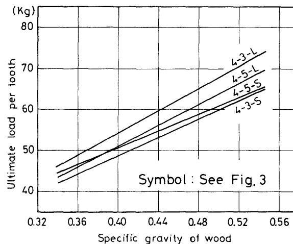
Fig. 8. Ultimate load per tooth as a function of specific gravity of wood. (In case of four rows type plate connectors)
