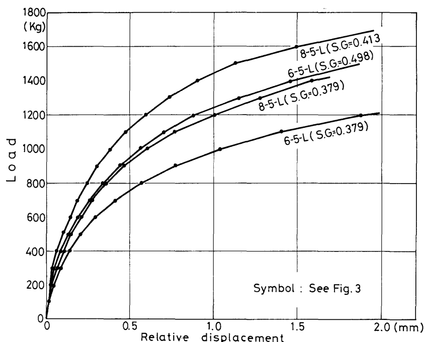
Fig. 13. Load-displacement curves of joints with six and eight rows type plate connectors.
