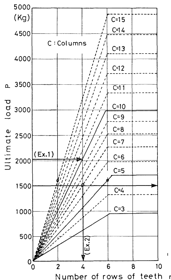
Fig. 14. Ultimate load of joints as a function of number of rows of teeth of plate connectors with a parameter of number of columns of teeth.
