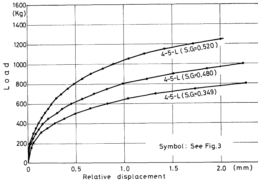
Fig. 9. Load-displacement curves of joints with four rows type plate connectors.
