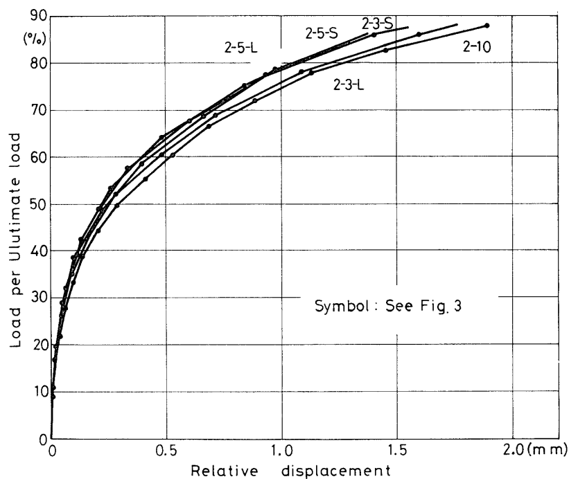
Fig. 6. Relation between fraction of individual ultimate load (load/ultimate load) and relative displacement of joints with two rows type plate connectors.
