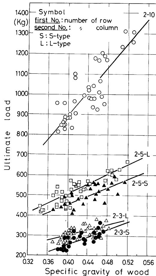
Fig. 3. Ultimate load of joints with two rows type plate connectors as a function of specific gravity of wood.
