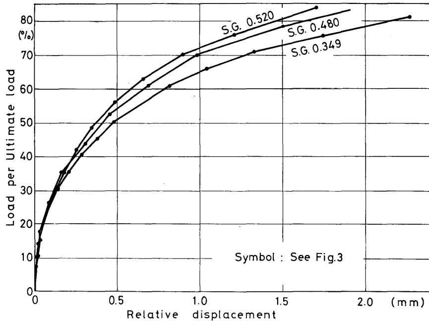
Fig. 10. Relation between fraction of individual ultimate load (load/ultimate load) and relative displacement of joints with four rows type plate connectors.
