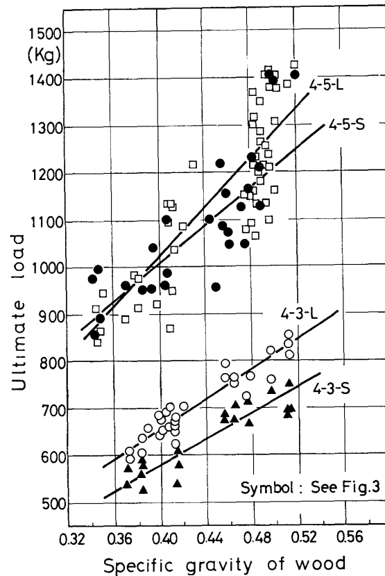
Fig. 7. Ultimate load of joints with four rows type of connectors as a function of specific gravity of wood.
