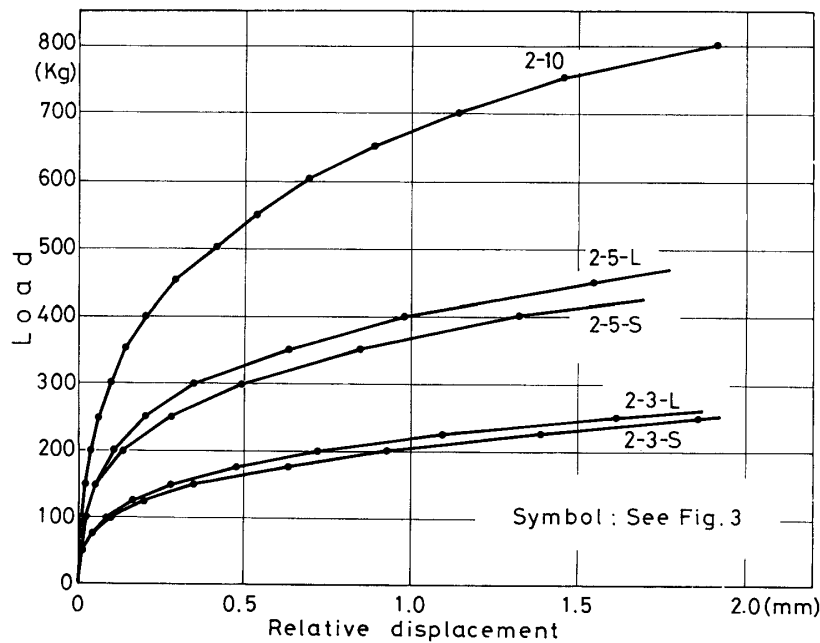
Fig. 5. Load-displacement curves of joints with two rows type plate connectors.
