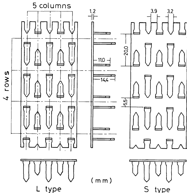
Fig. 1. An example of geometry and arrangement of teeth of a metal plate connector. (In case of 4 rows and 5 columns)
