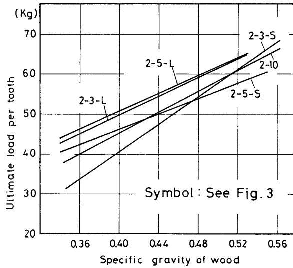
Fig. 4. Ultimate load per tooth as a function of specific gravity of wood. (In case of two rows type plate connectors)
