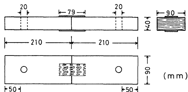
Fig. 2. An example of geometry of a joint specimen for static tensile test.
