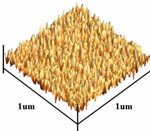
Figure 4-30(b). O 1500 V, 5 \times 10^{16} ions
