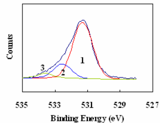
Figure 5-15(b). XPS O 1s of GZO
