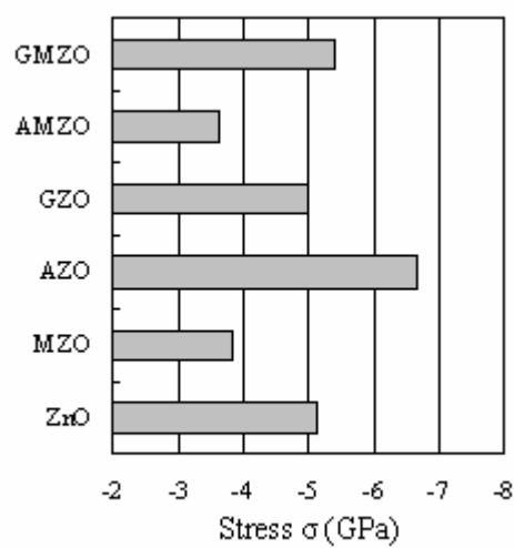
Figure 5-12 (b). Stress \sigma of TCOs
