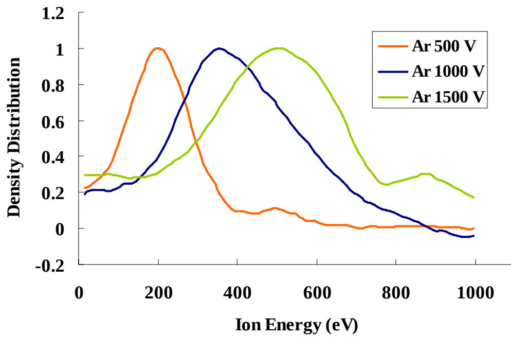
Figure 2-15. Ion energy and Density distribution
