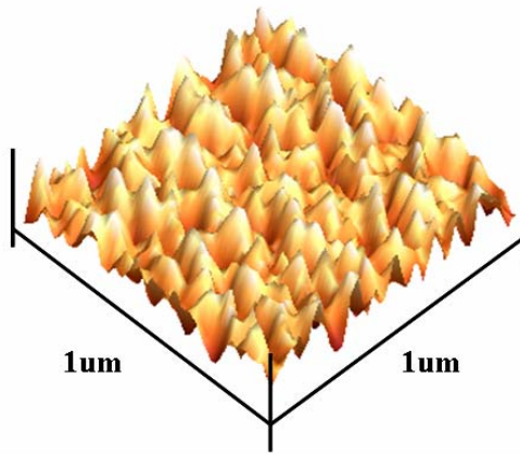
Figure 4-31(b). Ar 1000V, 1 \times 10^{16} ions
