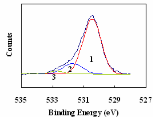
Figure 5-16(b). XPS O 1s of GMZO
