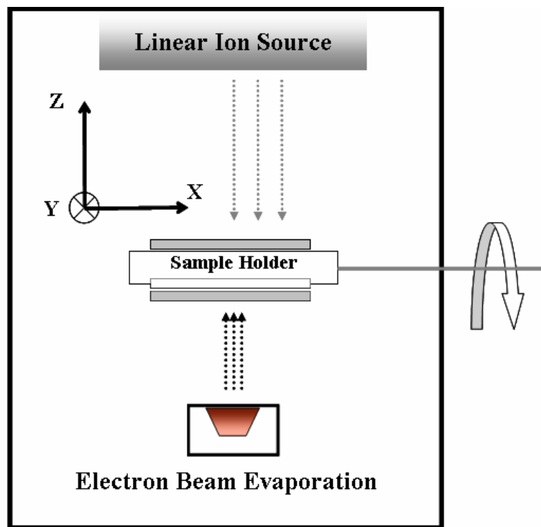
Figure 2-16. Linear ion source and electron beam evaporation chamber
