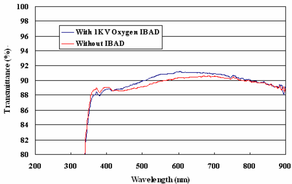
Figure 6-9. Light transmission of \text{SiO}_x with and without IBAD
