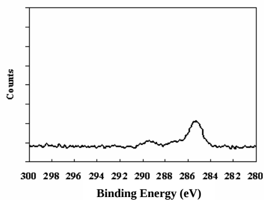
Figure 5-13(a). XPS C 1s before sputtering
