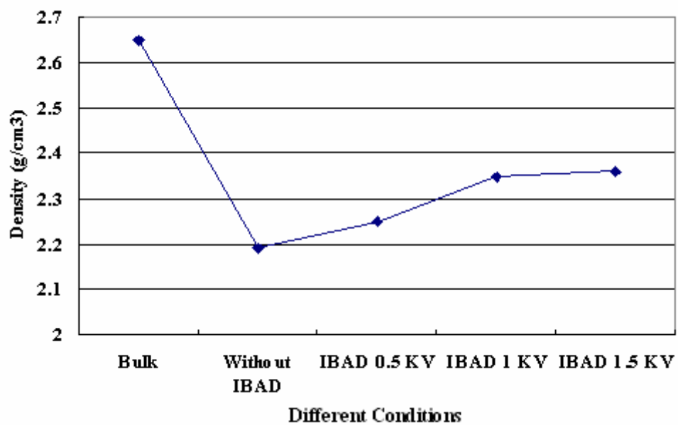
Figure 6-8. Density of \text{SiO}_x deposited at different conditions
