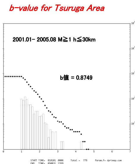
Fig. 5a The b-value for Fukui Earthquake fault region. 5b The b-value for Okuetsu region. 5c The b-value for Tsuruga region.
