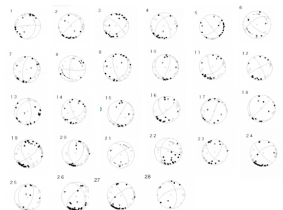
Fig.3 Fault plane solution which occurred at Reihoku region recently.
