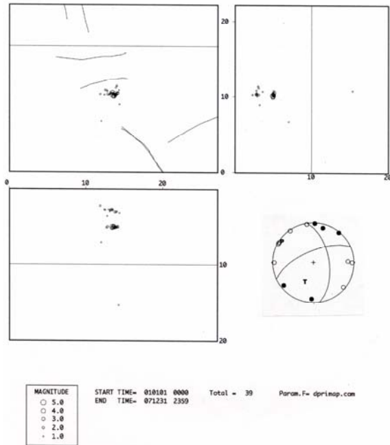
Fig2. Relocated hypocenter and fault plane solution.
