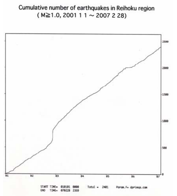
Fig.4a Epicenter of earthquake occurred at Reihoku region. 4b Cumulative number corresponds to 4a.
