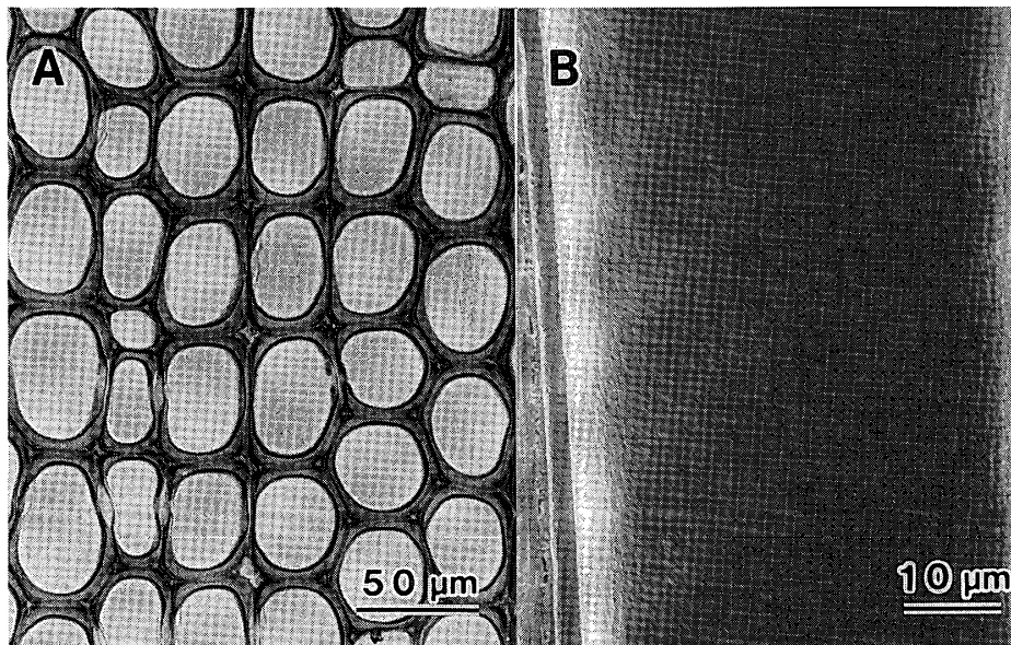
Fig. 1.3. Micrographs of the darkly colored wood portion of Podocarpus imbricatus . A : LM photograph of moderately thicker cell walls. B : SEM photograph of the S 3 layer with flat orientation of microfibrils.
