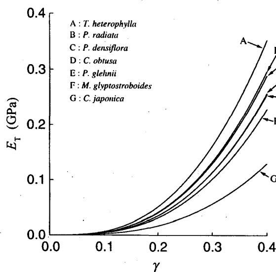
Fig. 4.6. Relationship between tangential Young's modulus E_T and specific gravity \gamma when cell wall thickness t changed.
