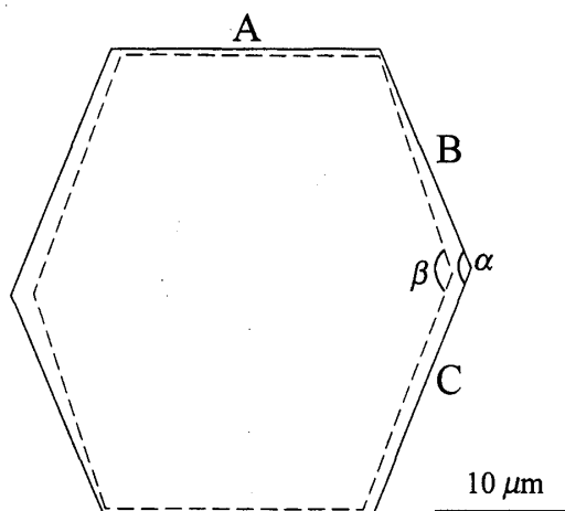
Fig. 2.15. A comparison of cell shapes in wet (solid line) and oven-dried (dotted line) conditions for the early wood tracheid of Chamaecyparis obtusa . \alpha : 135, \beta : 140.
