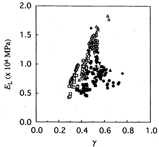
Fig. 1.8. Relationships between specific gravities ( \gamma ) and longitudinal Young's modulus ( E_L ) for all of the specimens examined. Legends: Refer to Fig. 1.5.
