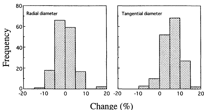
Fig. 2.7. Histograms for changes of radial and tangential lumen diameters of Agathis bornensis . Positive values show shrinkage and negative values show expansion.
