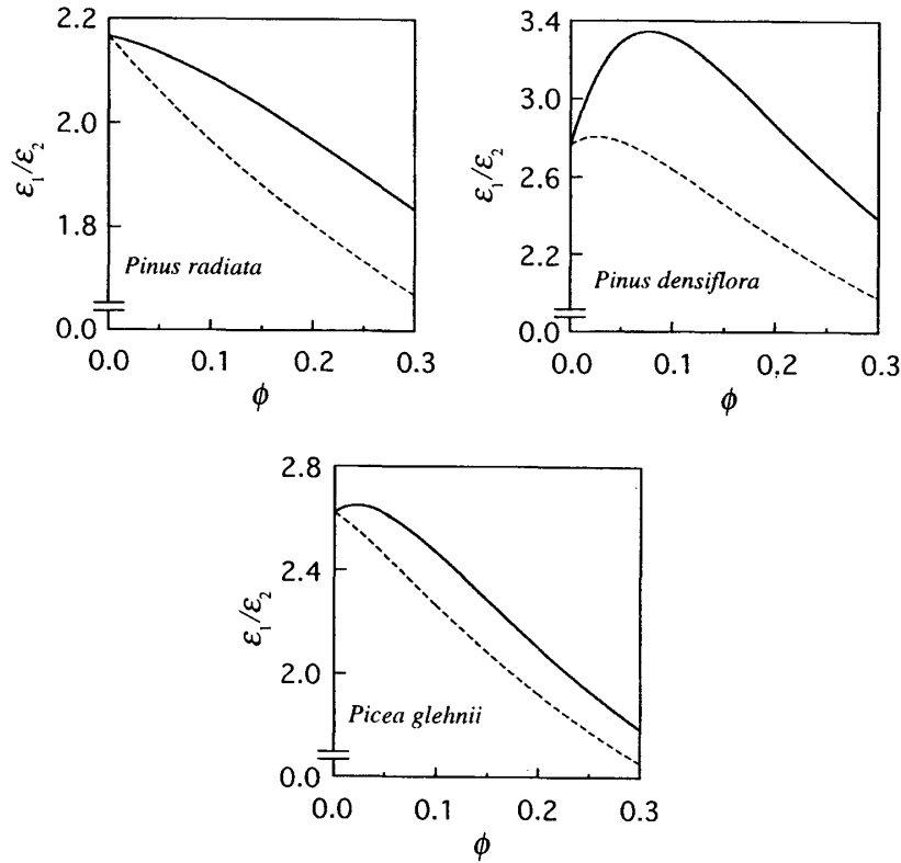
Fig. 3.8. Relationship between shrinkage anisotropy \epsilon_1/\epsilon_2 and late wood fraction \phi . Solid and dotted lines show the results with and without the interaction term C , respectively.
