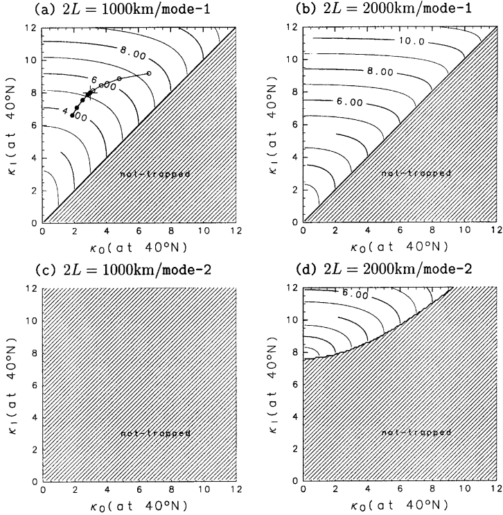
Fig. 4 The dependency of k on the variations of \bar{\kappa}_I and \bar{\kappa}_O . The 1st ((a) and (b)) and 2nd ((c) and (d)) modes for narrow ( 2L = 1000\text{km} , (a) and (c)) and wide ( 2L = 2000\text{km} , (b) and (d)) internal regions. See text for the details of the curve and symbols in (a).
