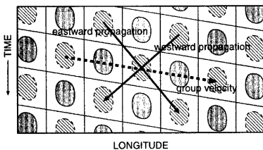
Fig. 14 A schematic longitude-time cross section representing the oblique checker pattern. The shaded areas and the hatched areas indicate southeries and northeries, respectively. The solid arrows show the westward and eastward phase propagations, while the dashed arrow shows the propagation of the wave packet, i. e., the group velocity.
