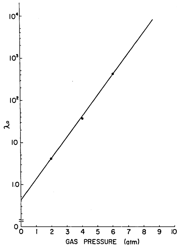
Fig.63 Estimated Values of \lambda_o as a Function of Gas Pressure
