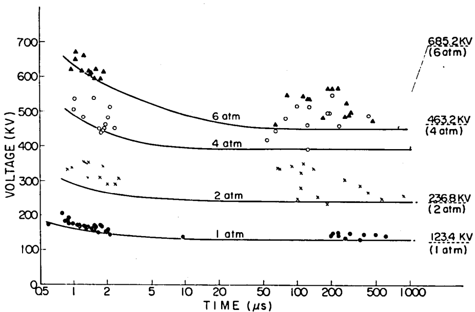
Fig.73(b) V-t Characteristics of Gap B ( d=2\text{cm} , u=0.606 , Negative)
