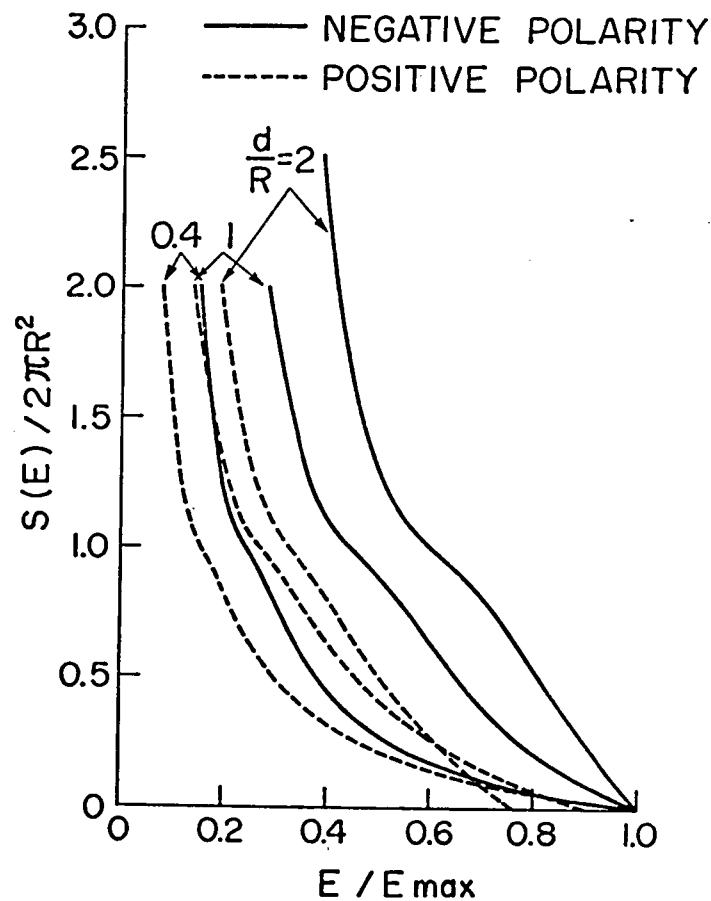
Fig.1-11 Examples of S^-(E) and S^+(E) for Rod-Rod Gaps
