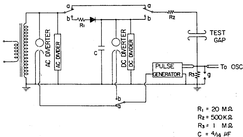
Fig.12 Schematic Diagram of the Test Circuit
