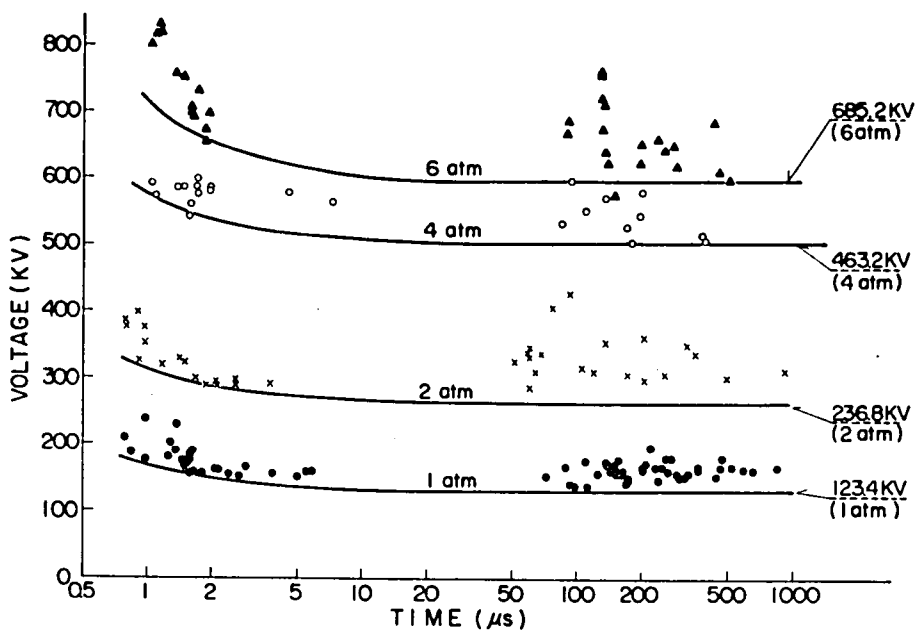
Fig.73(a) V-t Characteristics of Gap B ( d=2\text{cm} , u=0.606 , Positive)
