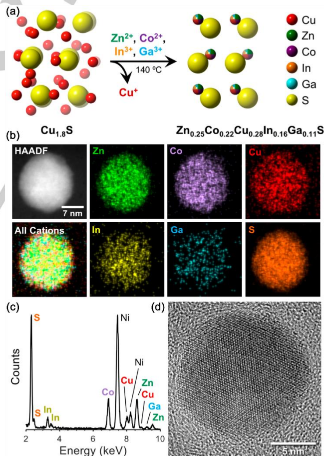
Figure 15. (a) Schematic of the formation of \text{Zn}_{0.25}\text{Co}_{0.22}\text{Cu}_{0.28}\text{In}_{0.16}\text{Ga}_{0.11}\text{S} NPs. (b) HAADF-STEM image and EDX elemental maps, (c) EDX spectrum, and (d) HRTEM image of \text{Zn}_{0.25}\text{Co}_{0.22}\text{Cu}_{0.28}\text{In}_{0.16}\text{Ga}_{0.11}\text{S} NPs. The Ni signal in (c) is from the TEM grid. (d) HRTEM image. Ref. [59] Copyright 2021, American Chemical Society.
