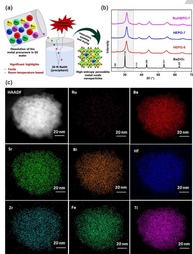
Figure 14. (a) Schematic of sonochemical-based synthesis of HEO NPs. (b) XRD patterns of \text{BaZrO}_3 , HEPO-5, 7, and Ru/HEPO-7. (c) EDX elemental maps of Ru/ \text{BaSrBi}(\text{ZrHfTiFe})\text{O}_3 (Ru/HEPO-7). ref. [56] Copyright 2020, Wiley-VCH Verlag GmbH & Co. KGaA.
