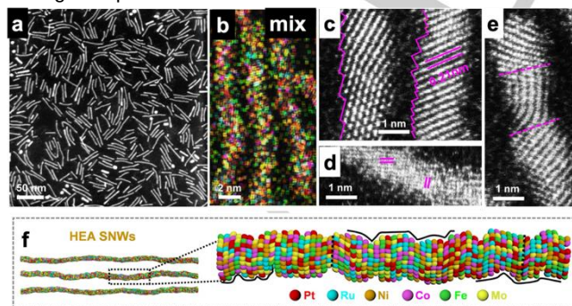
Figure 7. (a) HAADF-STEM image, (b) overlapped images of HAADF-STEM-EDX elemental maps, and (c-d) atomic-resolution STEM images, and (f) 3D atomic models of PtRuNiCoFeMo HEA SNWs. Reprinted with permission from ref. [28] Copyright 2021, Springer.
