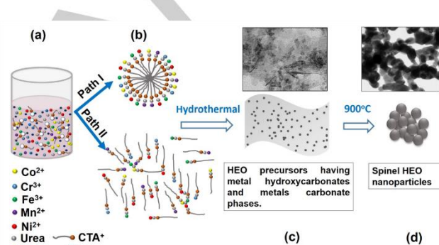
Figure 13. Formation mechanism of (Co, Cr, Fe, Mn, Ni) 3 O 4 NPs. (a) precursor solution, (b) two paths to form complex in the solution, (c) the formation of hydroxycarbonate and carbonate compounds during the hydrothermal treatment, (d) HEO NPs after heating. ref. [55] Copyright 2020, The Royal Society of Chemistry.
