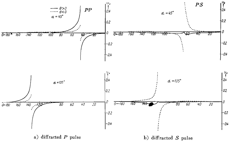
Fig. 6. The azimuthal distribution of the amplitude of displacement u_r, u_\theta of the diffracted pulse for the incidence of P pulse.
