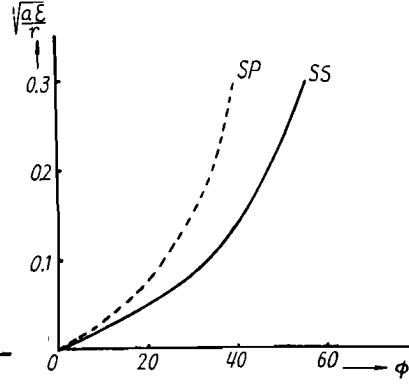
Fig. 8. \sqrt{a\epsilon}/r versus \phi for the incidence of P pulse.
