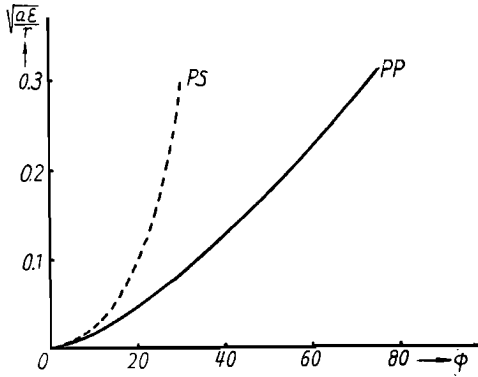
Fig. 8. \sqrt{a\epsilon}/r versus \phi for the incidence of P pulse.
