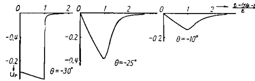
a) diffracted P pulse
