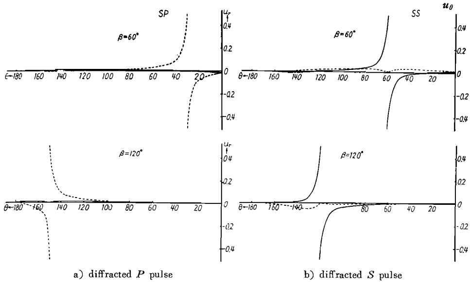
Fig. 7. The azimuthal distribution of the amplitude of displacement u_r , u_\theta of the diffracted pulse for the incidence of S pulse.
