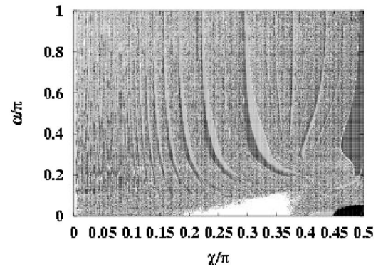
FIG. 3. Initial condition space of the DZV in D_{1/4} : \text{Li}^+ . Dark gray represents the electron-1 escape. Bright gray represents the electron-2 escape. Black represents the forbidden region ( E > 0 ). White represents the trapped trajectory.
