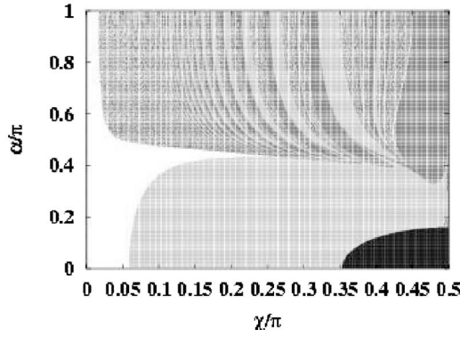
FIG. 1. Initial condition space of the DZV in D_{1/4} : \text{H}^- . Dark gray represents the electron-1 escape. Bright gray represents the electron-2 escape. Black represents the forbidden region ( E > 0 ). White represents the trapped trajectory.
