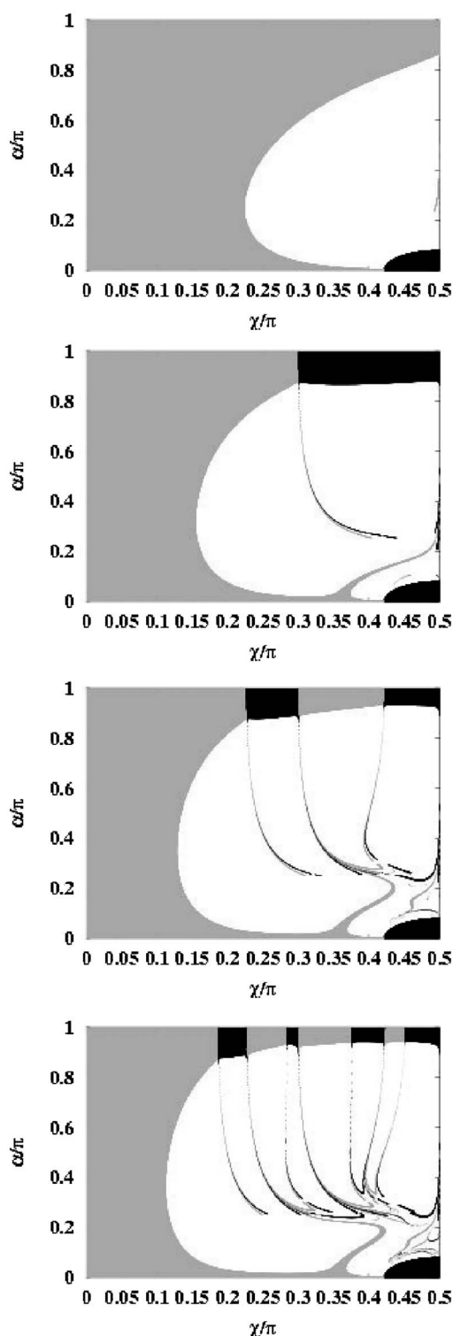
FIG. 5. Classification of the initial condition space D_{1/4} for He: (a) n_{\min}=1 , (b) n_{\min}=2 , (c) n_{\min}=3 , and (d) n_{\min}=4 . We set R=10^{-3} . S_0 (white), S_1 (black), S_2 (gray), S_3 (dark gray), and S_4 (none). The black region in lower right corner is a forbidden region ( E \geq 0 ).
