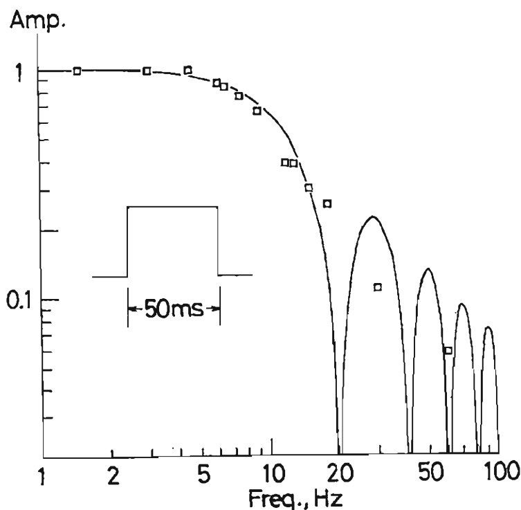
Fig. 3. Comparison of the measured spectrum with the theoretical one for a rectangular wave with duration time of 50 m sec.
