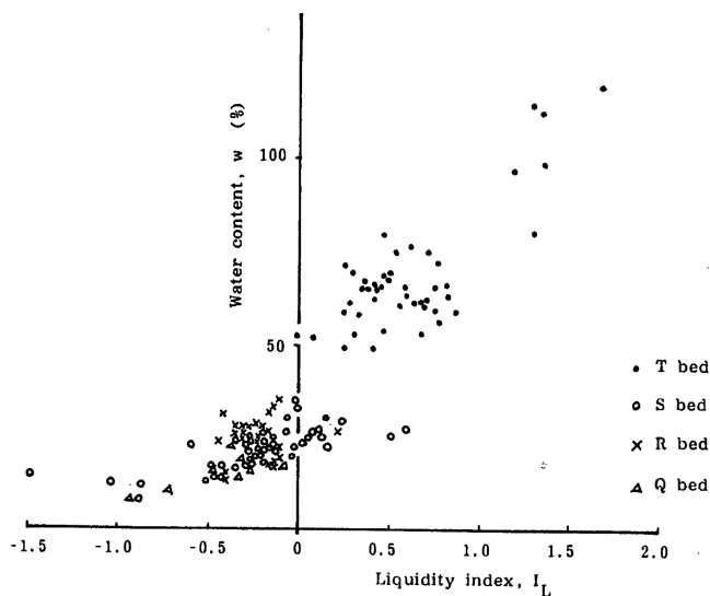
Fig. 6 Liquidity index versus natural water content of Lake Biwa deposit.
