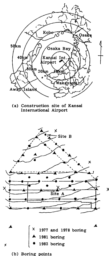
Fig. 10 Construction site of Kansai International Airport and its boring points.
