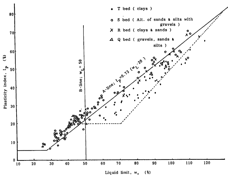
Fig. 5 Plastic chart of Lake Biwa deposit.
