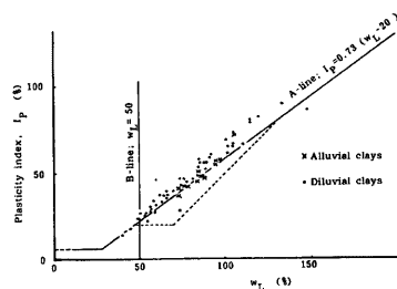
Fig. 12 Plastic chart of off shore samples.
