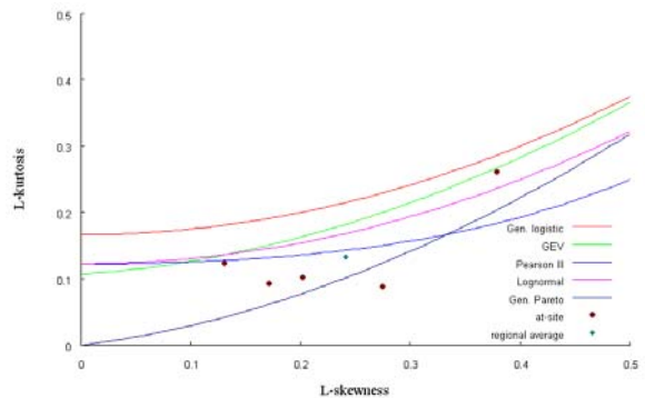
Fig. 8 L-moment ratio diagram for region 2.
