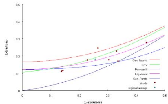
Fig. 7 L-moment ratio diagram for region 1.
