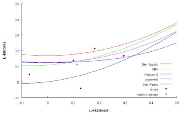
Fig. 11 L-moment ratio diagram for region 5.
