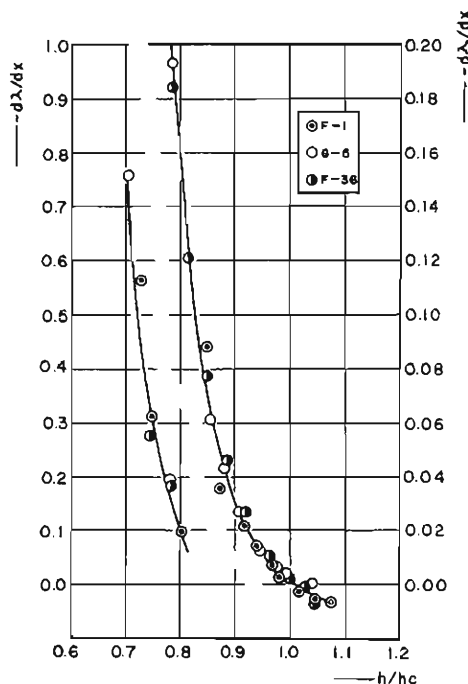
Fig. 2.3 Variation of d\lambda/dx against the flow depth.
