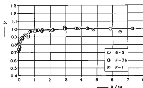
Fig. 2.2 Variation of \lambda along the channel.
