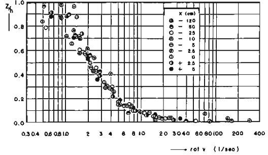
Fig. 4.2 Vertical distribution of vorticity.
