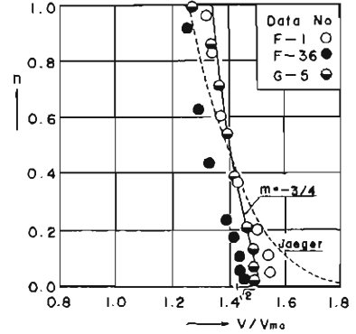
Fig. 4.4 Velocity distribution at the brink.
