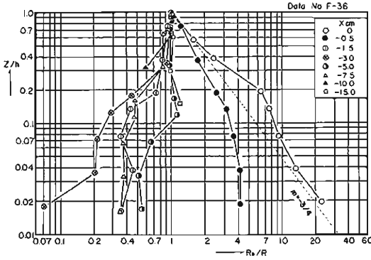
Fig. 4.3 Vertical distribution of curvature of streamlines.
