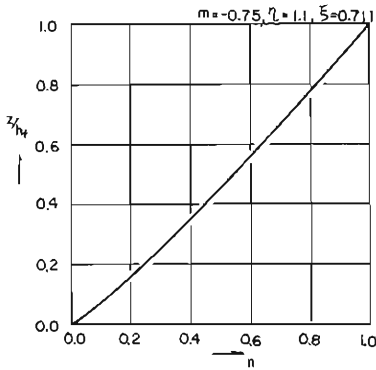
Fig. 4.5 Correlation curve between z and n . Fig. 4.6 Pressure distribution at the brink.
