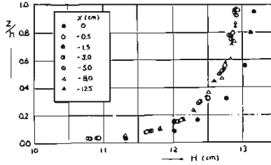
Fig. 4.1 Vertical distribution of energy.
