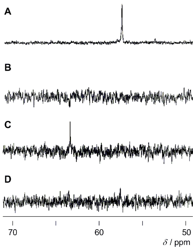
Figure 2. ^{13}\text{C} -NMR spectra of (A) ^{13}\text{C} -IQ-DTPA alone and (B, C, D) ^{13}\text{C} -IQ-Gd upon treatment with CYP450 reductase (10 \mu\text{g/mL} ) in the presence of \beta -NADPH (2 mM) at 37 °C in phosphate buffer (pH 7.4): (B) before treatment with reductase; (C) treated under hypoxic conditions for 1 h; (D) treated under aerobic conditions for 1 h.
