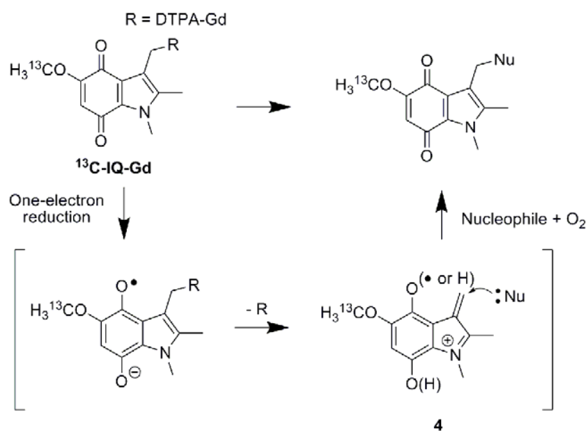
Figure 4. Plausible activation pathways of ^{13}\text{C-IQ-Gd} leading to elimination of DTPA-Gd unit followed by alkylation of the resulting iminium intermediate.
