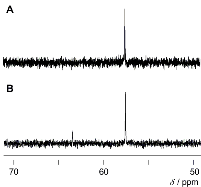
Figure 3. ^{13}\text{C} -NMR spectra of ^{13}\text{C} -IQ-OH (2 mM) (A) before and (B) after treatment with CYP450 reductase (10 \mu\text{g/mL} ) in the presence of \beta -NADPH (2 mM) at 37 ^{\circ}\text{C} for 1 h in hypoxic phosphate buffer (pH 7.4, 10% MeCN).
