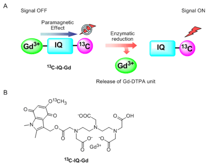
Figure 1. (A) Molecular design of ^{13}\text{C} -IQ-Gd as a probe for one-electron reduction by CYP450 reductase. (B) Chemical Structure of ^{13}\text{C} -IQ-Gd.
