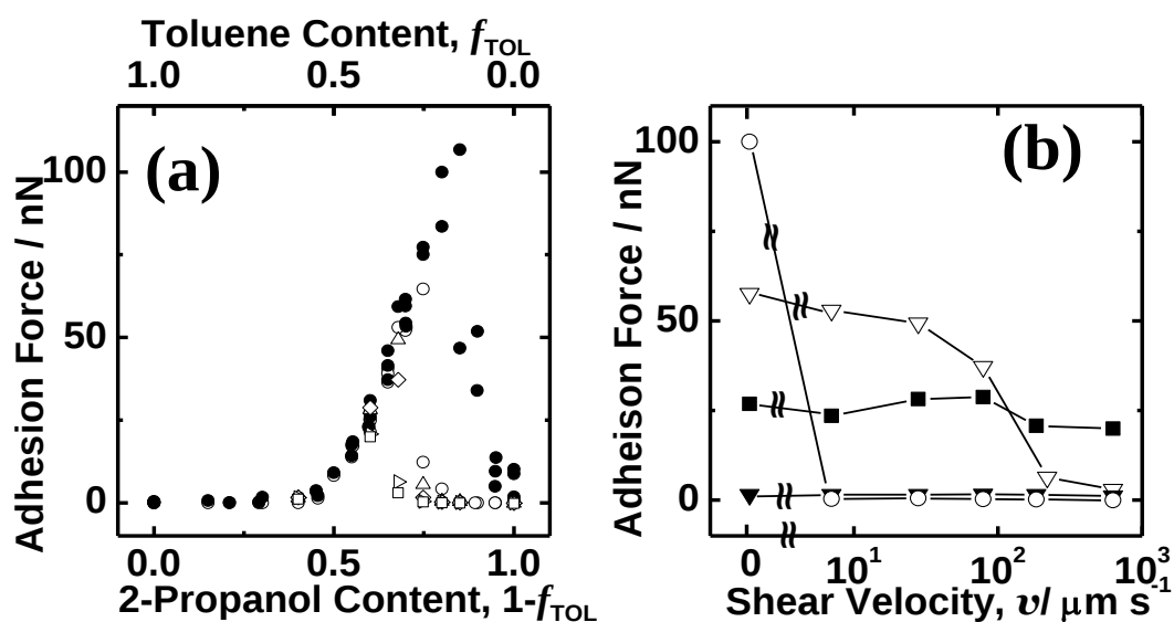
Figure 2-6. Plots of adhesion force between the PS brushes (samples 2 and 3 against PS-brush modified particle) as a function of (a) solvent composition f_{TOL} and (b) shear velocity v in toluene/2-propanol-mixed solvents; (a) v = 1000 ( \square ), 320 ( \diamond ), 100 ( \triangle ), 32 ( \circ ) 0 ( \bullet ) \mu\text{m/s} , and (b) f_{TOL}=0.6 ( \blacktriangledown ), 0.4 ( \blacksquare ), 0.3 ( \triangledown ), 0.2 ( \circ ). The PS-grafted SiP mounted on a rectangular-shaped cantilever was used as a probe.
