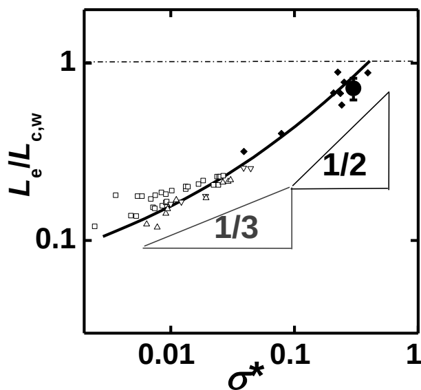
Figure 2-1. Plot of degree of stretching L_e/L_{c,w} vs dimensionless graft density \sigma^* of the PS brush (Sample 1) in toluene ( \bullet ). Other symbols reprocessed from the reference 4(b) show the data for some other polymer brushes in good solvents including the CPB of PMMA in toluene (small closed symbols).
