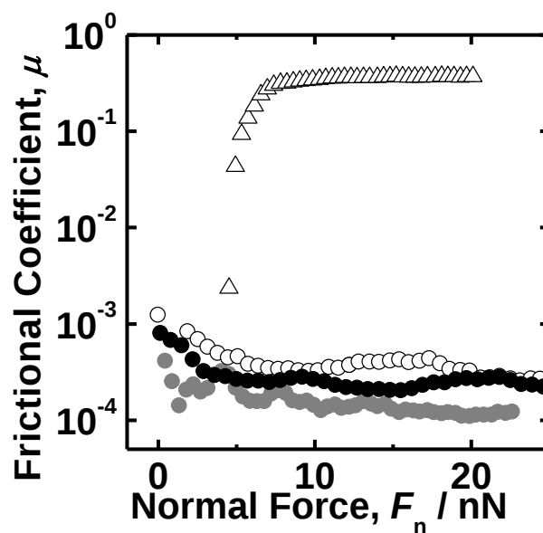
Figure 4-1. Plot of frictional coefficient \mu vs normal load F_n at shear velocity v of 6 \mu\text{m/s} for the SDPBs of PMMA ( \triangle , Wafer 1/Probe 1, the data was reprocessed from the reference 5), CPBs of PMMA ( \bullet , Wafer 1/Probe 1) and PS ( \circ , Wafer 1/Probe 1), and dissimilar CPBs of PMMA-PS ( \bullet , CPB of PS Wafer 1/CPB of PMMA Probe 1).
