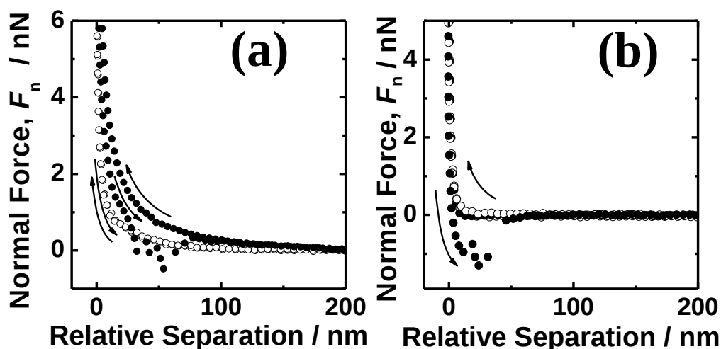
Figure 5-5. Approaching and retracting-mode force curve profiles measured between PHEA brushes and PPEGa brushes in (a) water ((●) PHEA Wafer 1/Probe 1 and (○) PPEGa Wafer 1/Probe 1) and in (b) 10^{-1} M NaCl aqueous solution ((●) PHEA Wafer 1/Probe 1 and (○) PPEGa Wafer 2/Probe 1).
