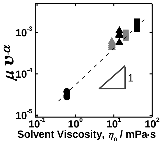
Figure 3-5. Plot of frictional coefficient normalized with shear velocity, \beta = \mu v^{-\alpha} , vs bulk solvent viscosity, \eta_0 , in toluene at 30 °C (●), DEME-TFSI at 30 °C (■) and 58 °C (▲), and EMI-TFSI at 30 °C (■) and 58 °C (▲).
