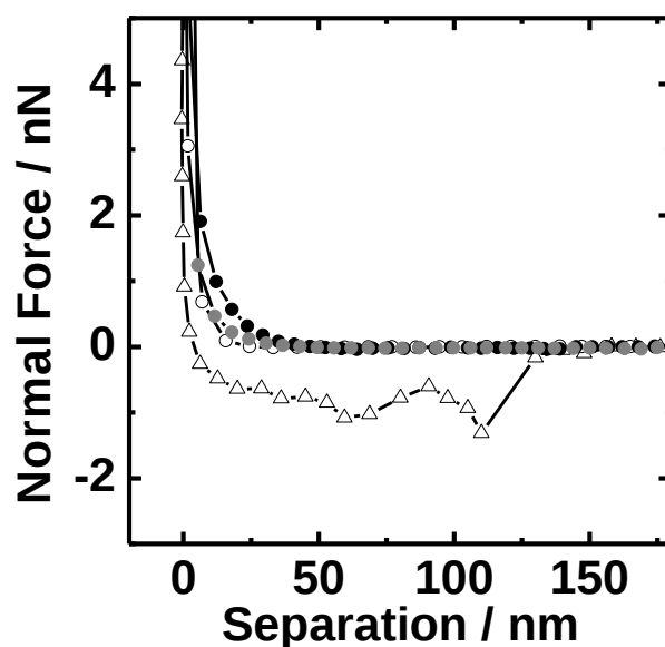
Figure 4-3. Typical retractive force curve profiles of SDPBs of PMMA ( \triangle , Wafer 1/Probe 1), CPBs of PMMA ( \bullet , Wafer 1/Probe 1) and PS ( \circ , Wafer 1/Probe 1), and dissimilar CPBs of PMMA-PS ( \bullet , CPB of PS Wafer 1/CPB of PMMA Probe 1).
