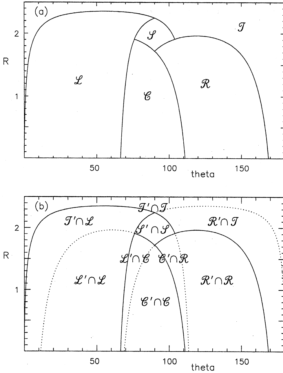
Figure 2: (a) Division of the surface of section. (b) Overlapping regions of the surface of section and its reverse.
