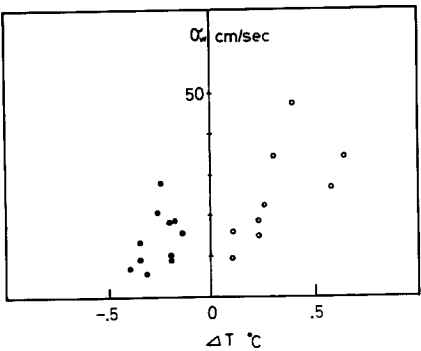
Fig. 10 \sigma_w inside ( \Delta T > 0 ) and outside ( \Delta T < 0 ) of the thermals.
