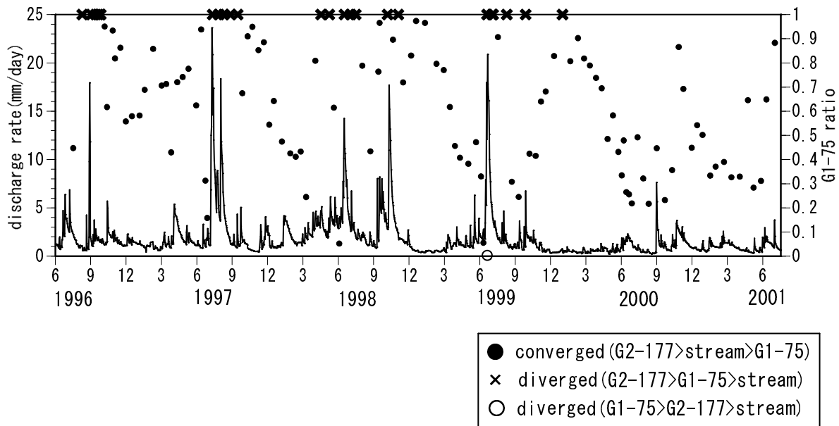
Figure 5.4 Temporal variations of SGW shallow layer contributions
