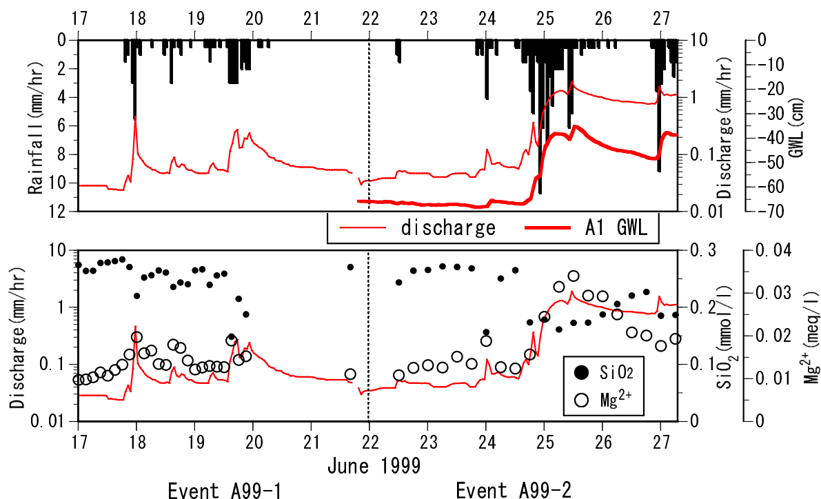
Figure 6.6 Temporal variations in rainfall, discharge rate, groundwater levels and \text{SiO}_2 and \text{Mg}^{2+} concentrations of the Akakabe catchment
