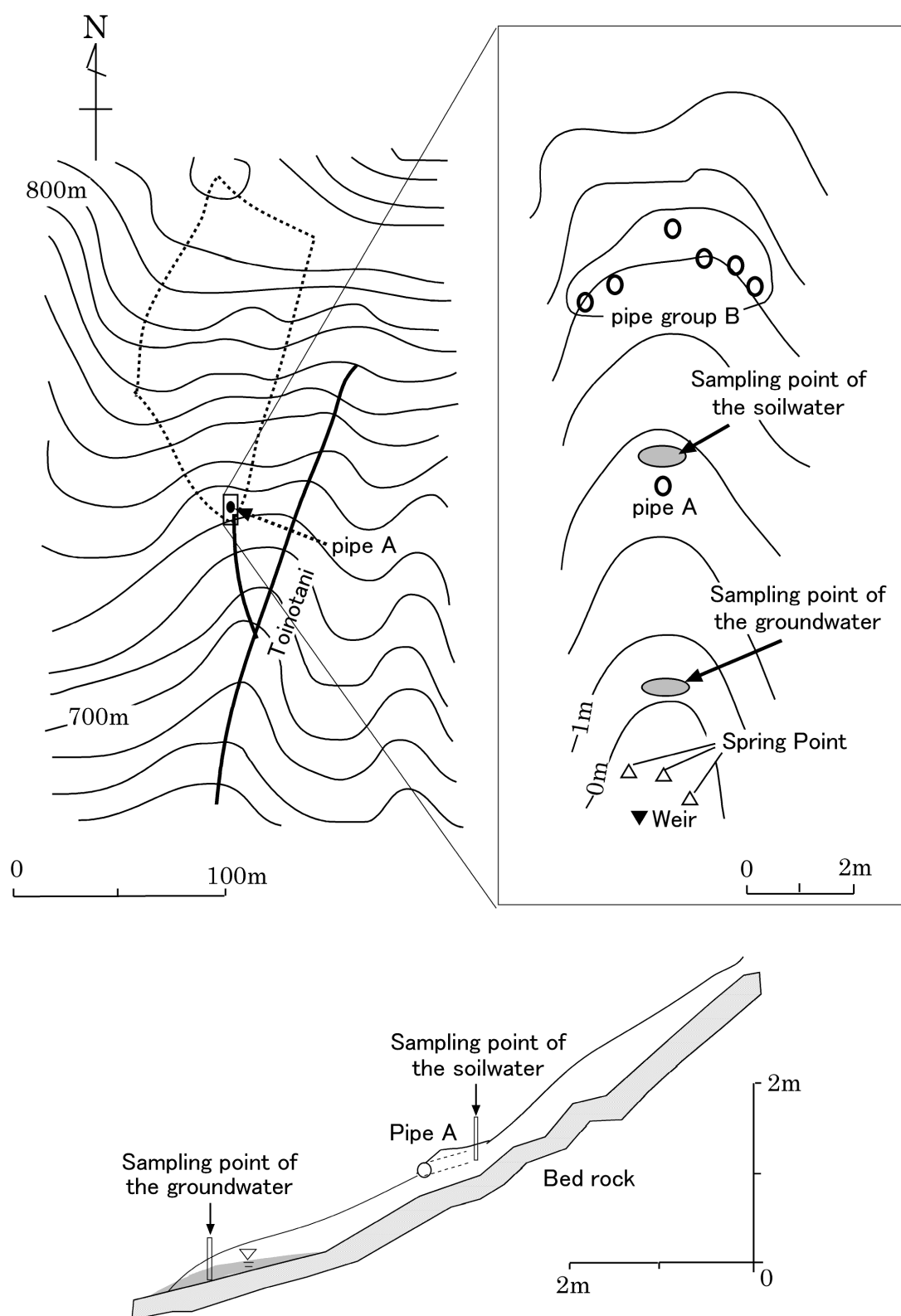
Figure 2.12 Ground surface topography and a longitudinal section of the Toinotani catchment
