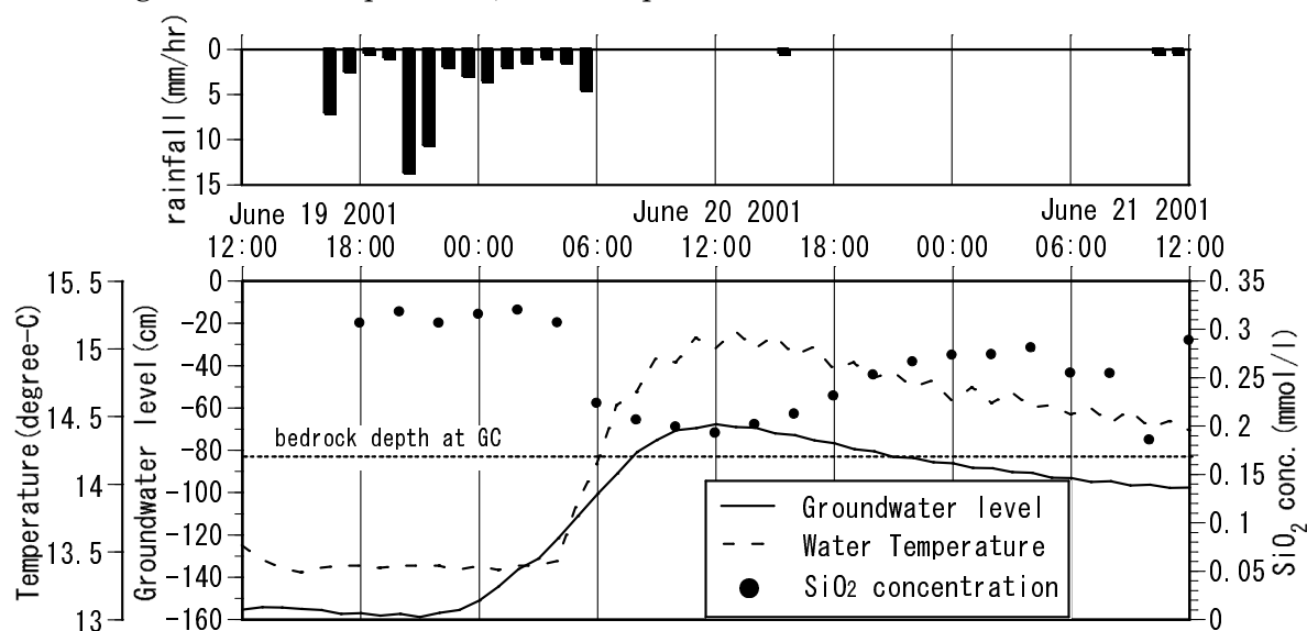
Figure 4.3 Short-term variations of \text{SiO}_2 concentrations and groundwater levels and groundwater temperature at GC
