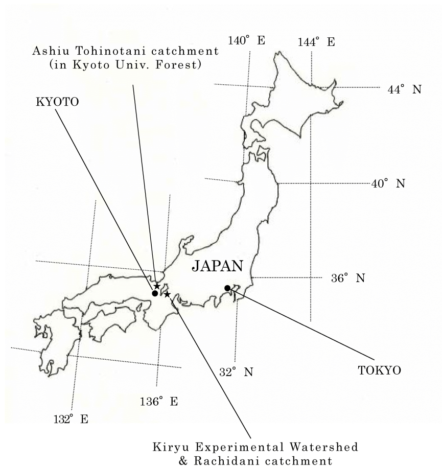
Figure 2.1 Locations of the study sites
