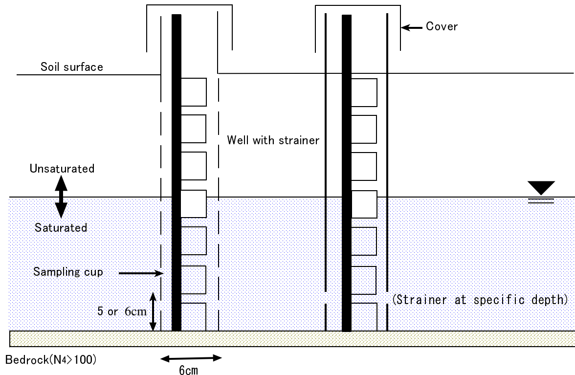
Figure 2.13 The structure of the observation wells (Maximum rise well)
