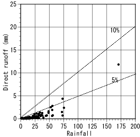
Figure 3.5 Direct runoff ratio in the Matsuzawa catchment
