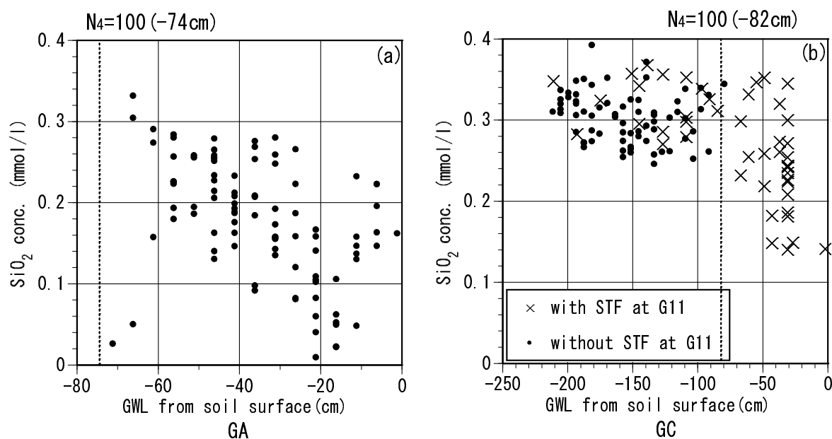
Figure 4.2 Relationship of groundwater levels and \text{SiO}_2 concentrations at GA and GC note: "STF" denotes the subsurface storm flow.
