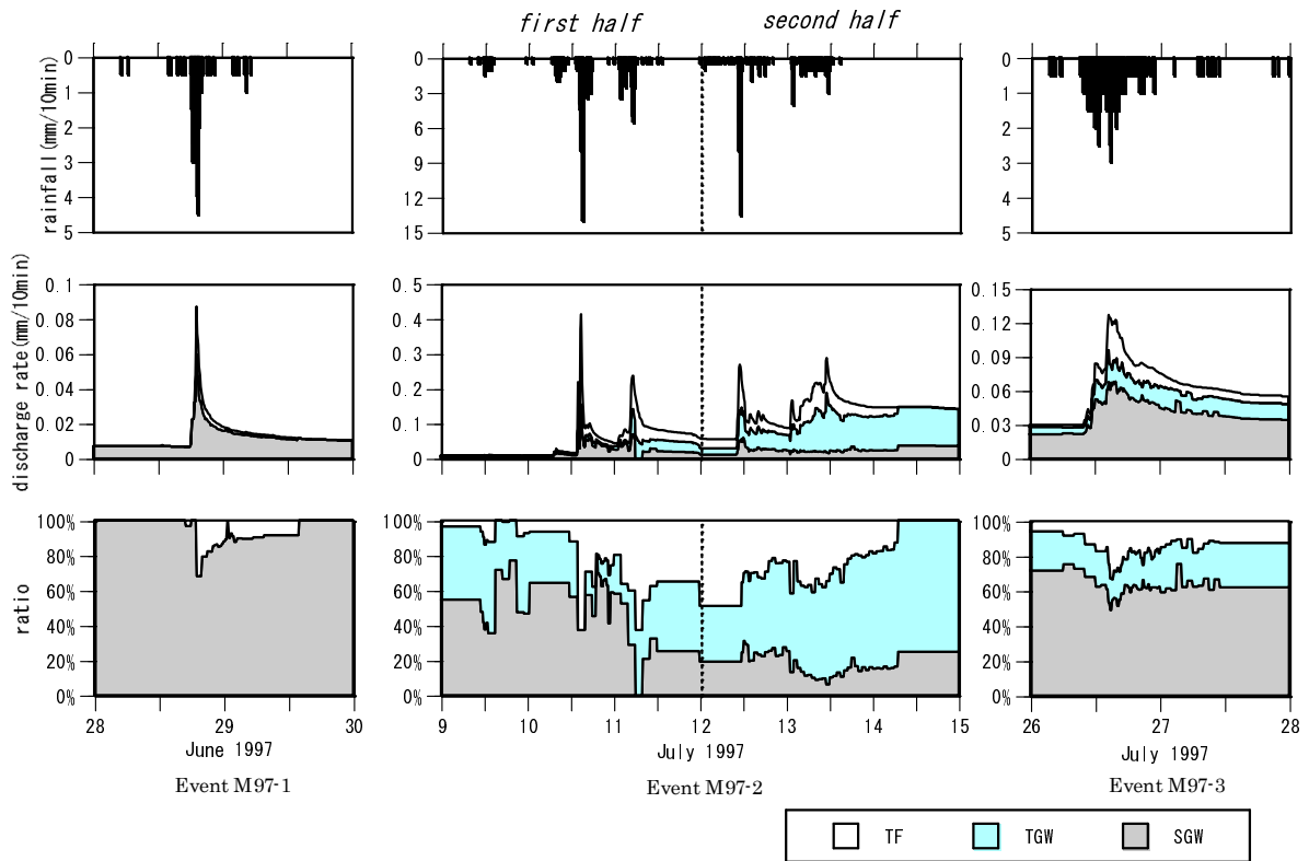
Figure 6.5 Hydrograph separations
