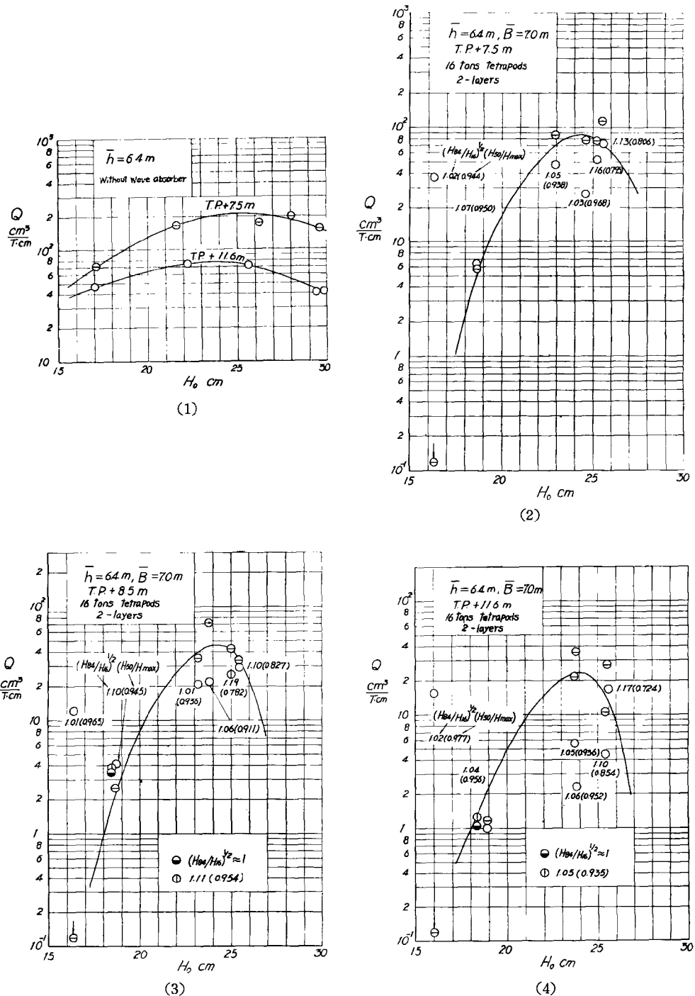
Fig. 3 Relations between rate of wave overtopping and deep-water wave height for case of 16 tons tetrapods ( \bar{h}=6.4m )
