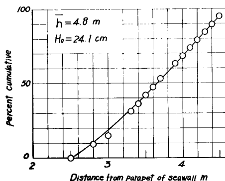
Fig. 9 An example of cumulative frequency diagrams of plunging points of waves
