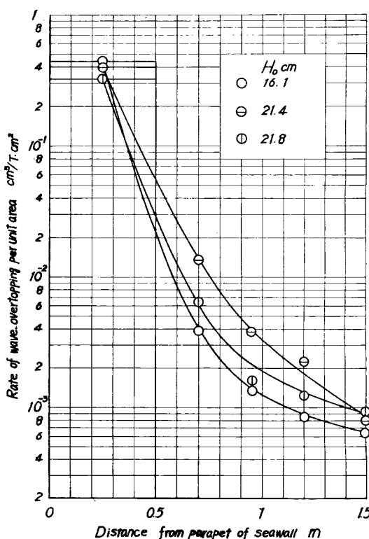
Fig. 7 Horizontal distribution of rate of wave overtopping ( \bar{h}=6.4 m)
