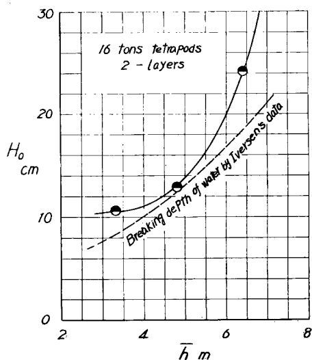
Fig. 13 Relation between deep-water wave height for maximum rate of wave overtopping and water depth in front of seawall
