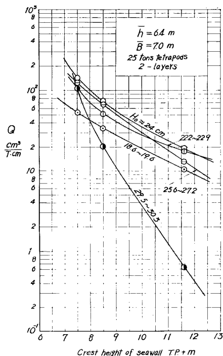
Fig. 10 Relations between rate of wave overtopping and crest height of seawall for case of 25 tons tetrapods ( \bar{h}=6.4 m)
