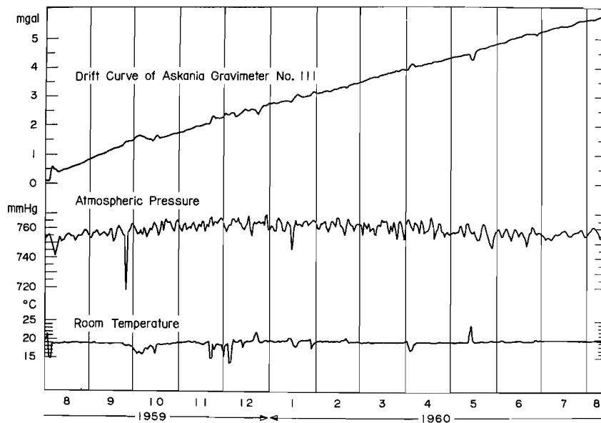
Fig. 3.1. Drift curve of the Askania gravimeter No. 111 determined by Pertzev's method and the changes of atmospheric pressure and room temperature.
