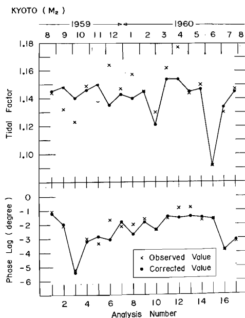
Fig. 3.2. Tidal factor of gravity and phase lag.
