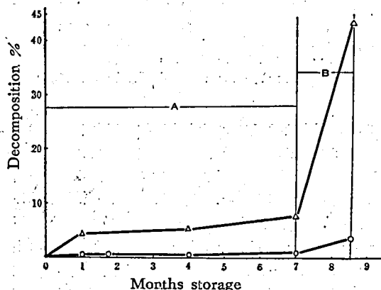
Fig.1. Effect of storage temperature and stabilizer on the decomposition of malathion dust formulation. A: at room temp. B: at 40°, —○— Clay, —△— Clay+Stabilizer 0.7% ( C_{11}H_{23}O(CH_2CH_2O)_7H )
