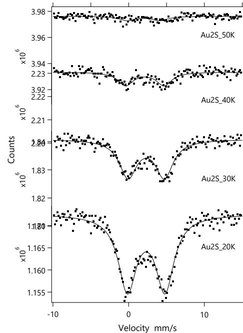
Fig. 1. Mössbauer spectra of \text{Au}_2\text{S} at each temperature. The ratio of the vertical axis is the same.
