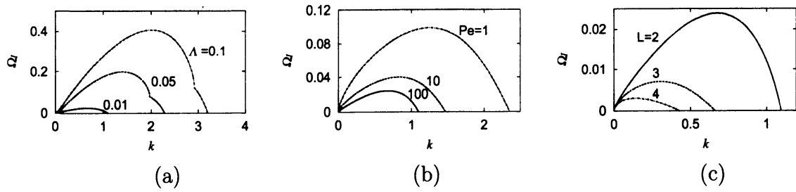
図 2: 実波数 k に対する時間増幅率の変化 ( Re = 100 , Wb = 100 , E_w = 1 ): (a) Pe = 100 , L = 2 , \Lambda = 0.1, 0.05, 0.01 , (b) \Lambda = 0.01 , L = 2 , Pe = 1, 10, 100 , (c) \Lambda = 0.01 , Pe = 100 , L = 2, 3, 4 .
