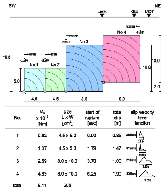
Fig. 7 The derived four asperity model and each slip velocity function, together with the source specifications (after Matsushima and Kawase, 2000).
