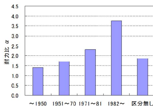
Fig. 15 Average yield strength ratios of wooden houses with different construction ages derived from the damage survey by local governments after the 1995 Hyogo-ken Nanbu earthquake (after Yoshida et al., 2004).
