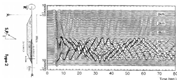
Fig. 2 Time-domain responses on the surface of a double trapezoidal basin (on the left) for a vertically incident SH wave with the predominant period of 4 s, which corresponds to the fundamental resonant period of the basin (after Kawase and Aki, 1989).
