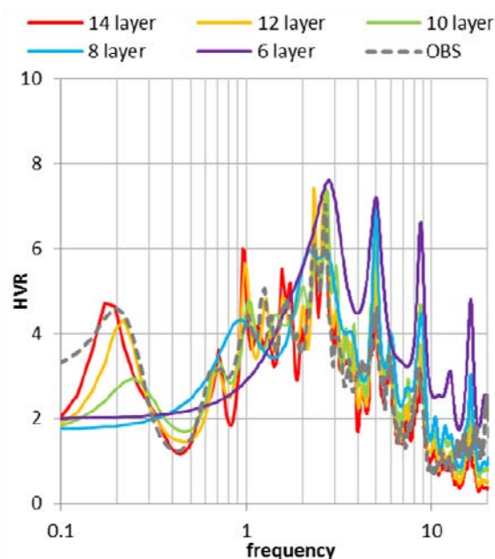
Fig. 19 Comparison of 1D theoretical earthquake HVSRs for the velocity model identified at MYG006 with different numbers of layers from the top as a parametric study. A broken line shows the observed HVSR. The original inverted structure has 14 layers down to the seismological bedrock (after Kawase et al., 2018).
