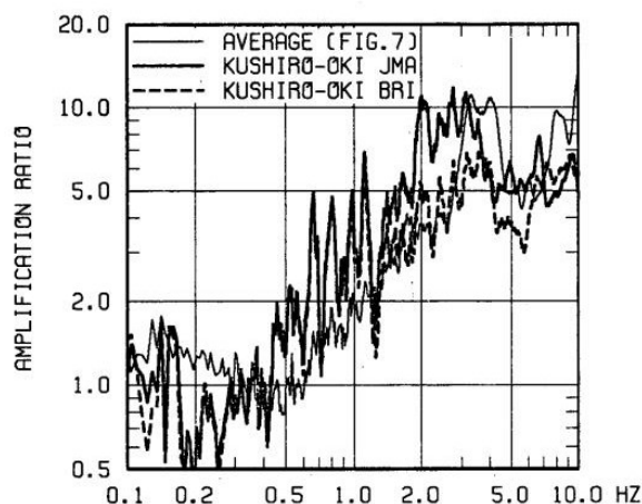
Fig. 3 Site amplification factors separated at the Kushiro site by the two different sensors (after Kawase, 1994).
