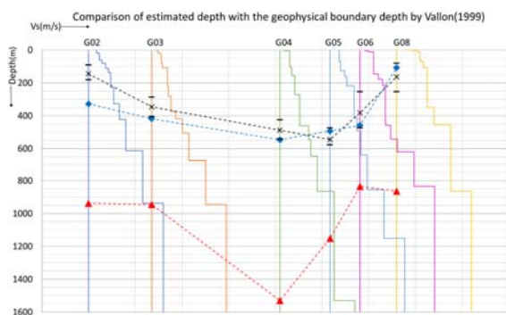
Fig. 23 A sectional view of the inverted velocity structures along a perpendicular line of the northeastern part of the Grenoble Basin. Black crosses with dotted lines are those of the geological boundary from gravity measurements.
