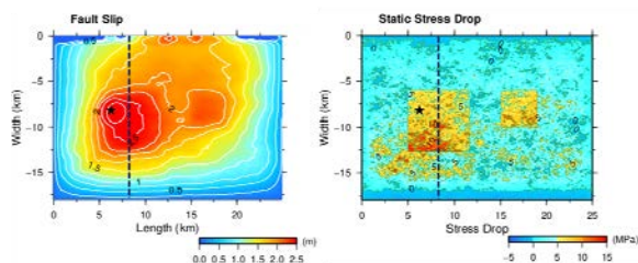
Fig. 16 Slip distribution as a result of dynamic rupture simulation on the left with two distinctive asperities on the right (after Manpo et al., 2018). Dark blue broken lines are the measurement line for Fig.17.
